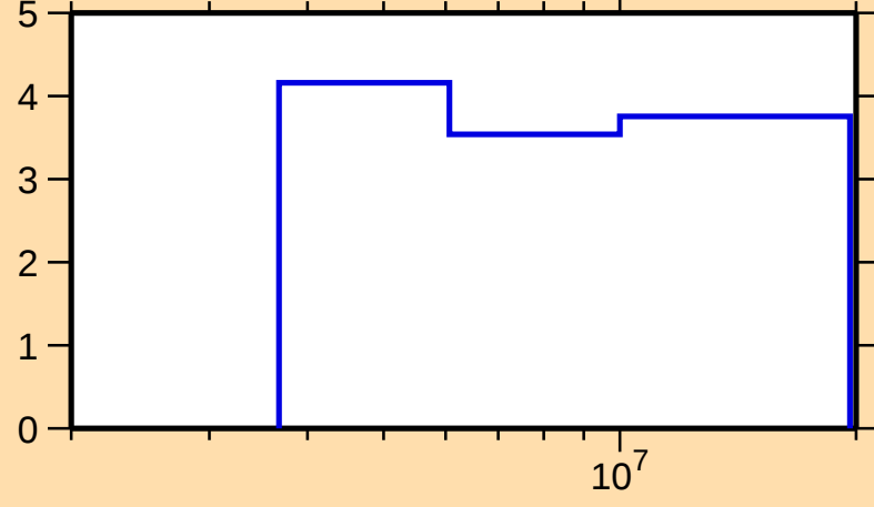
\Delta\sigma/\sigma vs. E for ^{116}\text{Ag}(n,\text{nonel.})
