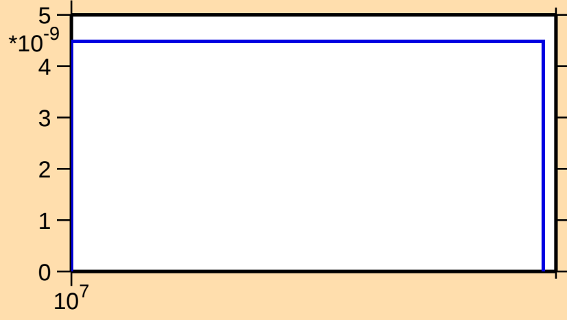
\sigma vs. E for ^{116}\text{Ag}(n,nt)
