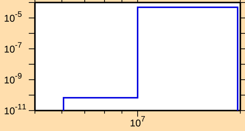
\sigma vs. E for ^{116}\text{Ag}(n,t)
