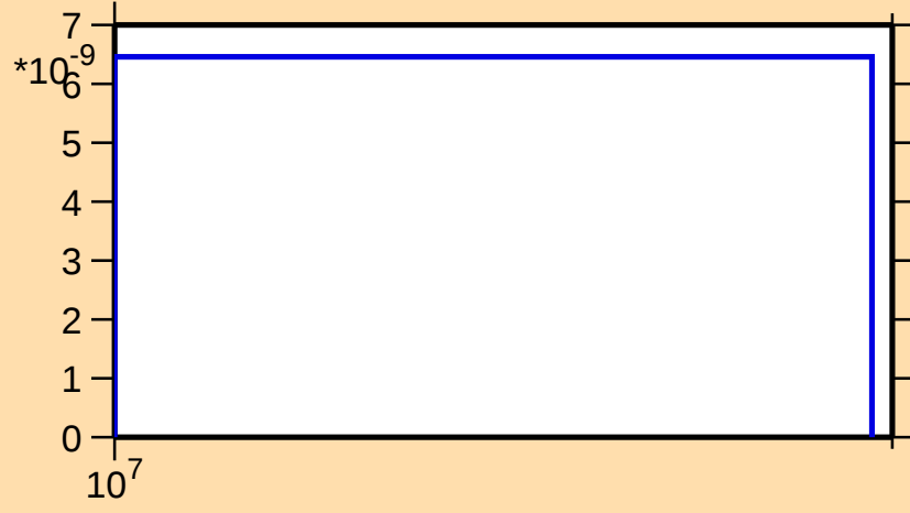
\sigma vs. E for ^{116}\text{Ag}(n,2np)
