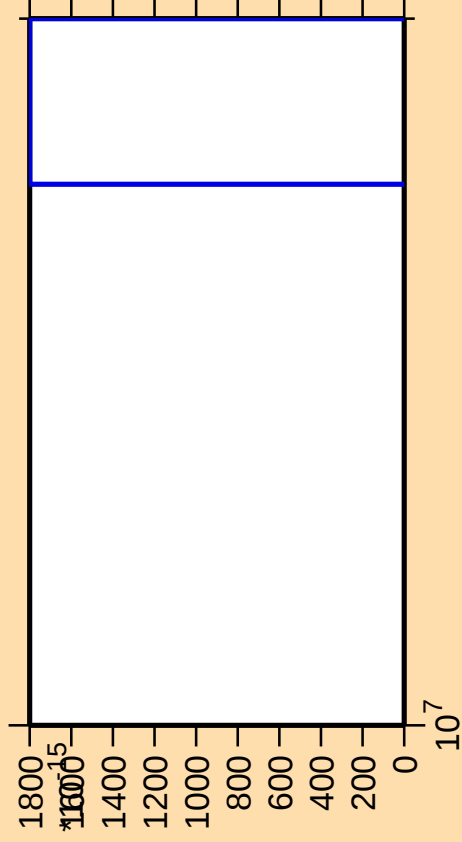
\Delta\sigma/\sigma vs. E for ^{119}\text{Ag}(\text{mt } 11)
