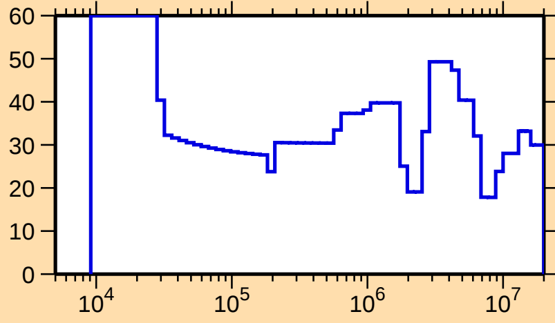
\Delta\sigma/\sigma vs. E for ^{119}\text{Ag}(n,\text{el.})
