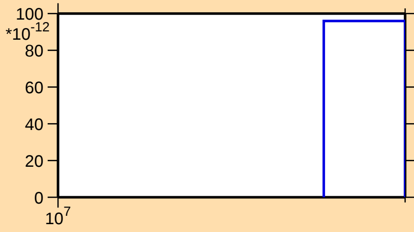
\sigma vs. E for ^{119}\text{Ag}(n,2np)
