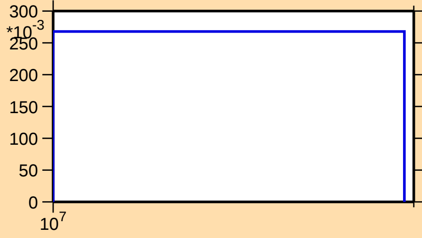
\sigma vs. E for ^{119}\text{Ag}(n,3n)
