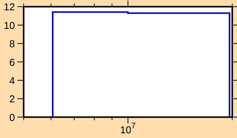
\Delta\sigma/\sigma vs. E for ^{119}\text{Ag}(n,\text{nonel.})
