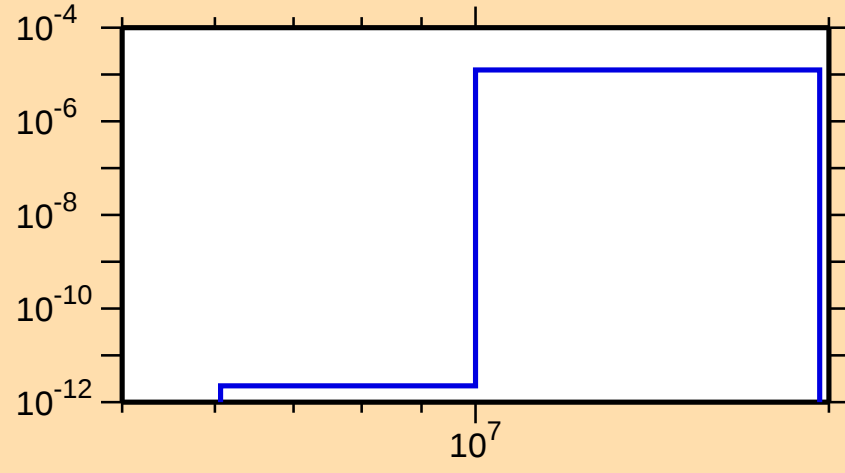
\sigma vs. E for ^{119}\text{Ag}(n,\alpha)
