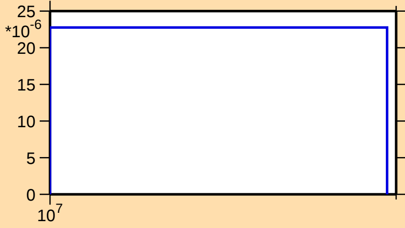
\sigma vs. E for ^{119}\text{Ag}(n,np)
