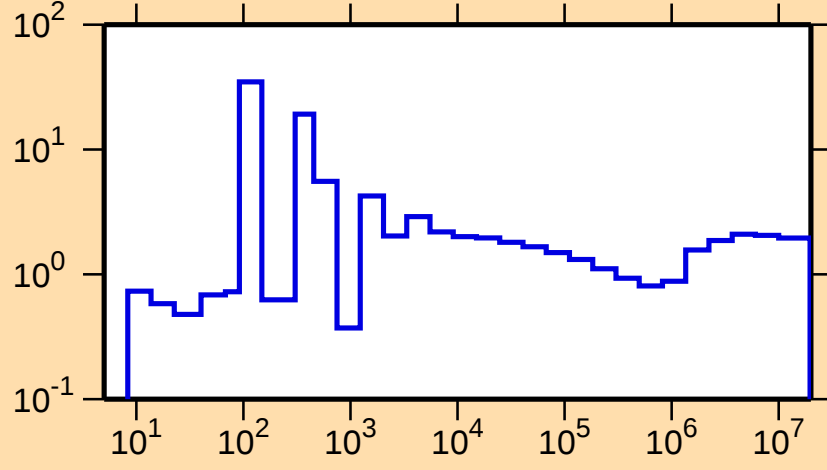
\sigma vs. E for ^{119}\text{Ag}(n,\text{nonel.})
