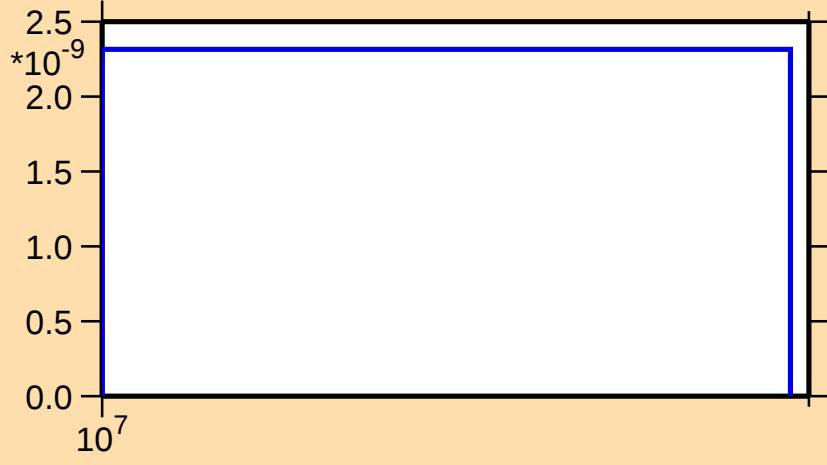
\sigma vs. E for ^{119}\text{Ag}(n,nt)
