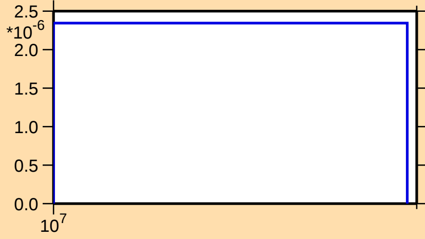
\sigma vs. E for ^{119}\text{Ag}(n,t)
