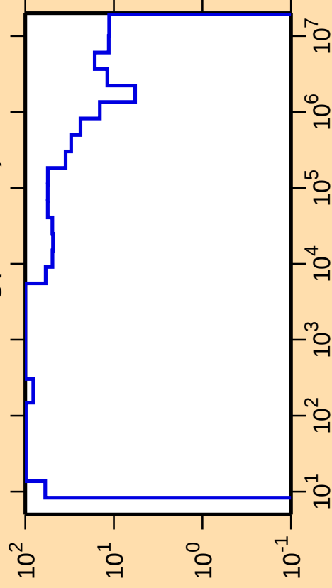
\Delta\sigma/\sigma vs. E for ^{119}\text{Ag}(n,\text{nonel.})
