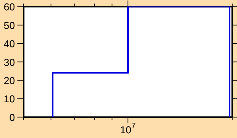
\Delta\sigma/\sigma vs. E for ^{119}\text{Ag}(n,n\text{cont.})
