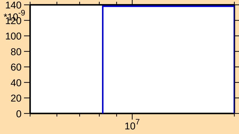
\sigma vs. E for ^{119}\text{Ag}(n,n\alpha)
