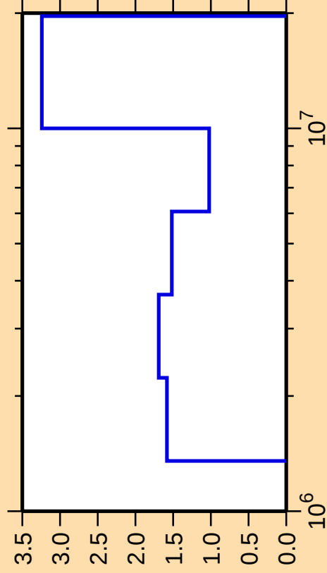
\Delta\sigma/\sigma vs. E for ^{29}\text{Al}(\text{n,inel.})
