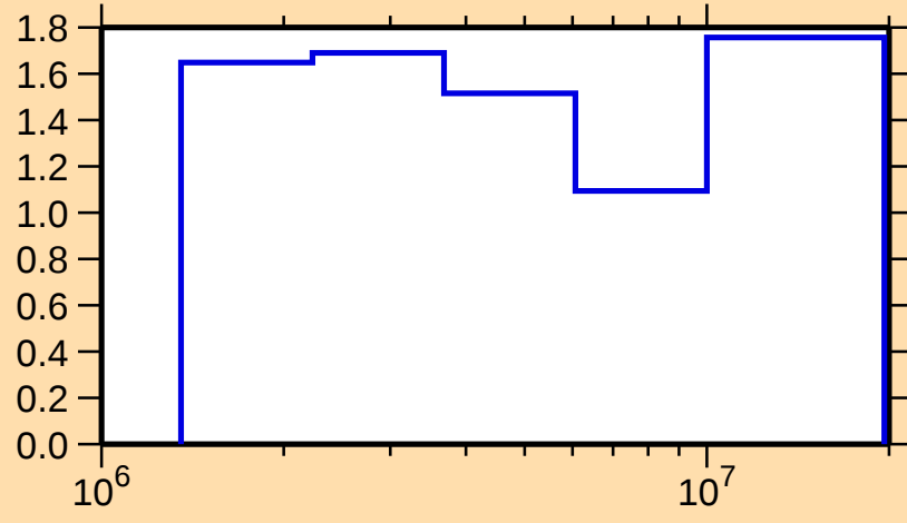
\Delta\sigma/\sigma vs. E for ^{29}\text{Al}(\text{n,nonel.})
