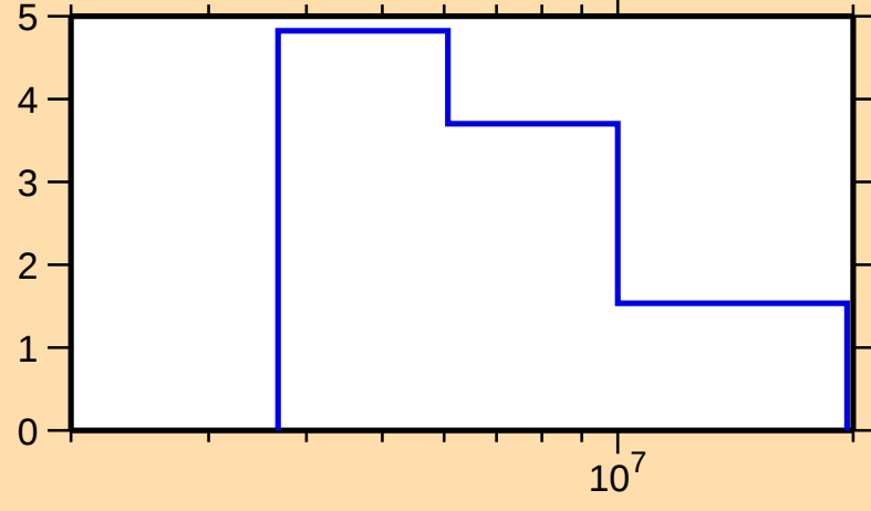
\Delta\sigma/\sigma vs. E for ^{29}\text{Al}(\text{n},\text{el.})
