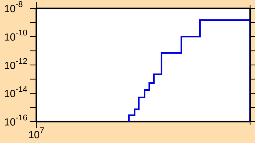
\sigma vs. E for ^{235}\text{Am}(n,2np)
