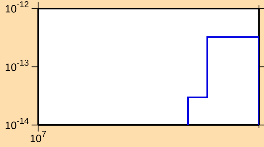
\sigma vs. E for ^{235}\text{Am} (mt 45)
