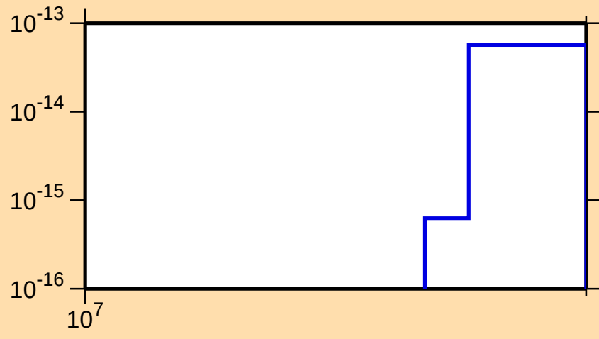
\sigma vs. E for ^{235}\text{Am}(n,3n\alpha)
