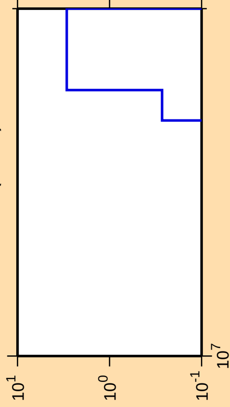
\Delta\sigma/\sigma vs. E for ^{235}\text{Am} (mt 45)
