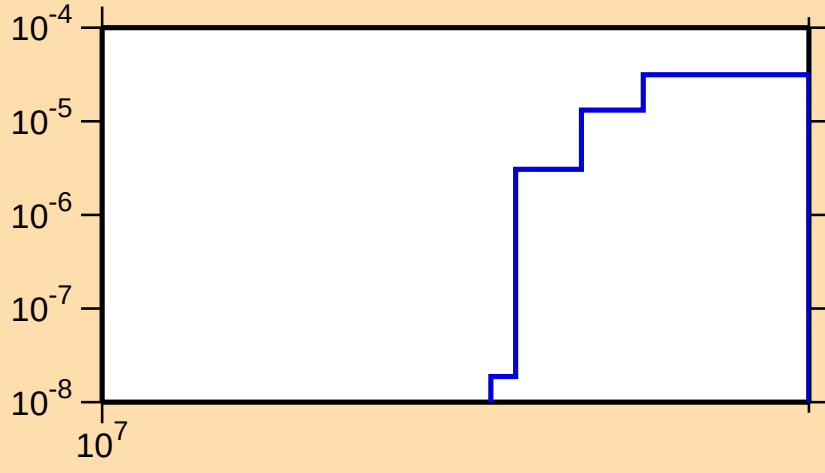
\sigma vs. E for ^{235}\text{Am}(n,3n)
