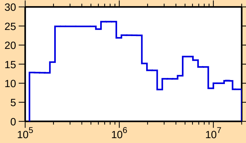
\Delta\sigma/\sigma vs. E for ^{235}\text{Am}(n,\text{el.})
