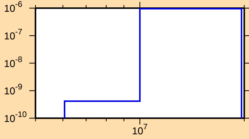
\sigma vs. E for ^{235}\text{Am}(n,np)
