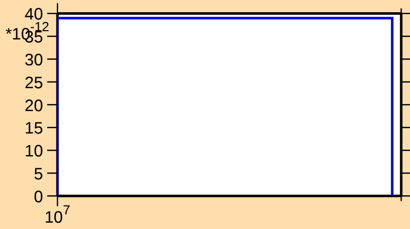
\sigma vs. E for ^{235}\text{Am}(n,\text{nt})
