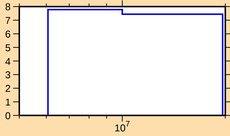
\Delta\sigma/\sigma vs. E for ^{235}\text{Am}(n,\text{nonel.})
