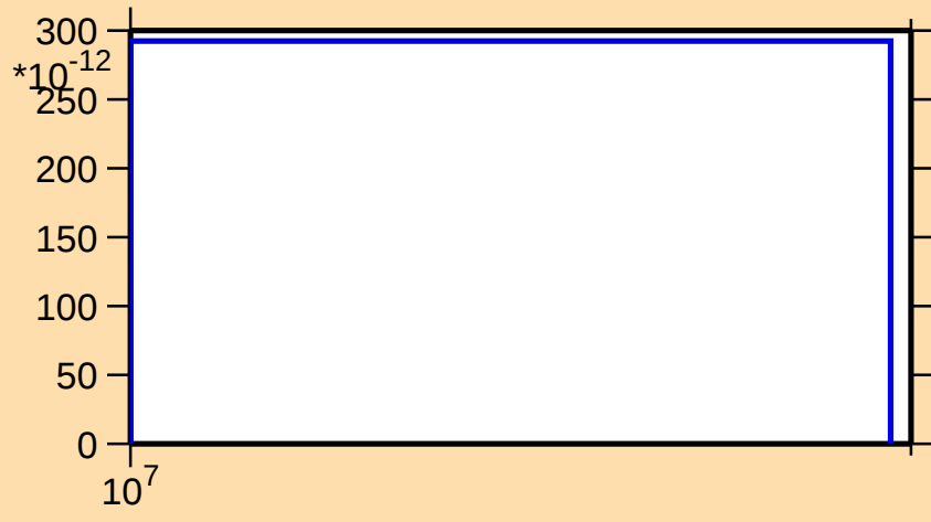
\sigma vs. E for ^{235}\text{Am}(n,\text{He3})
