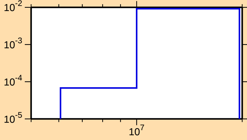
\sigma vs. E for ^{235}\text{Am}(n,2n)
