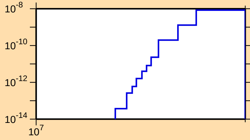
\sigma vs. E for ^{236}\text{Am}(n,2np)
