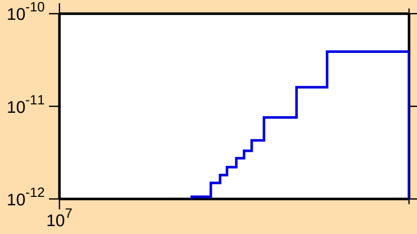
\sigma vs. E for ^{236}\text{Am}(n,p\alpha)
