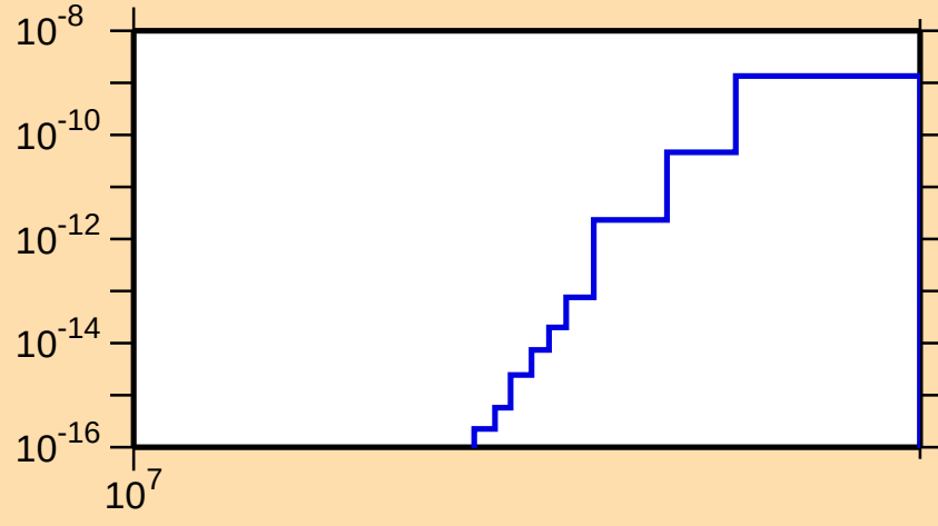
\sigma vs. E for ^{236}\text{Am}(n,nt)
