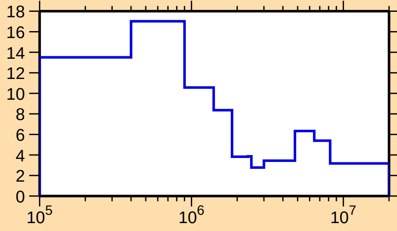
\Delta\sigma/\sigma vs. E for ^{236}\text{Am}(n,\text{tot.})
