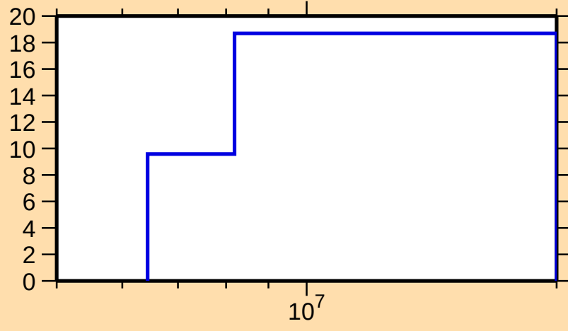
\Delta\sigma/\sigma vs. E for ^{236}\text{Am}(n,\text{el.})
