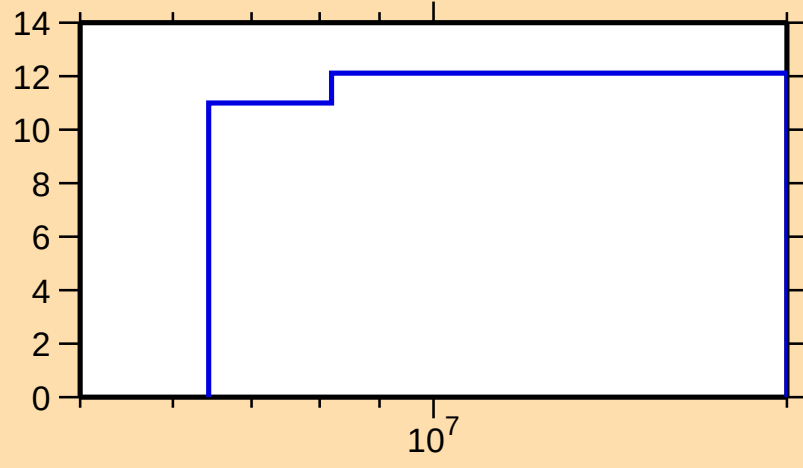
\Delta\sigma/\sigma vs. E for ^{236}\text{Am}(n,\text{nonel.})
