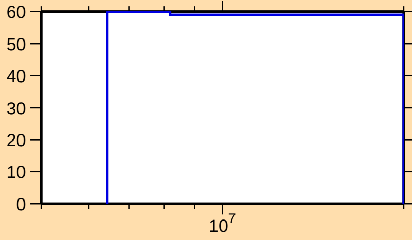
\Delta\sigma/\sigma vs. E for ^{236}\text{Am}(n,2n)
