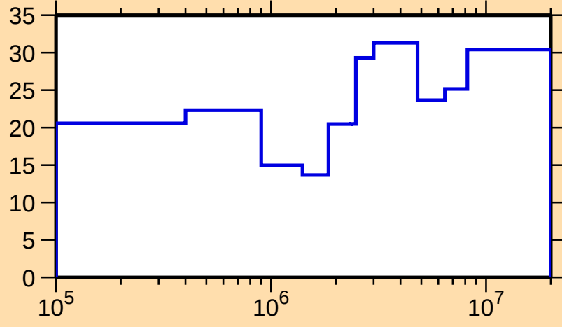
\Delta\sigma/\sigma vs. E for ^{236}\text{Am}(n,n_1)
