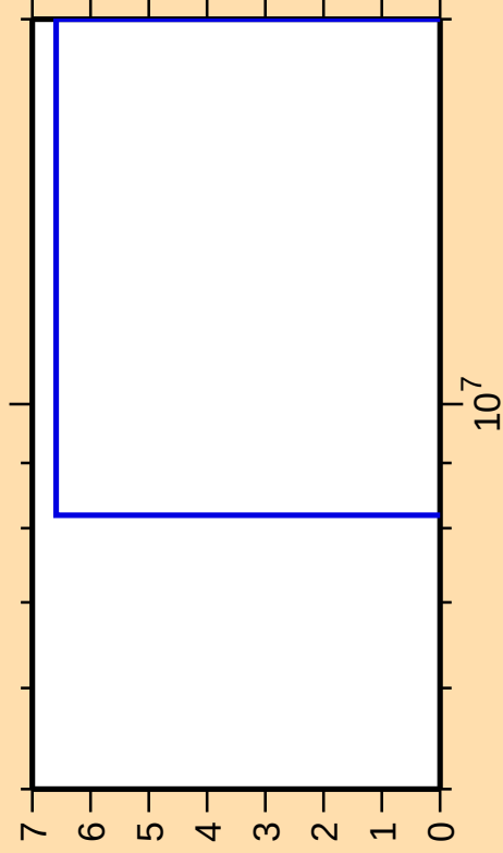
\Delta\sigma/\sigma vs. E for ^{236}\text{Am}(n,nt)
