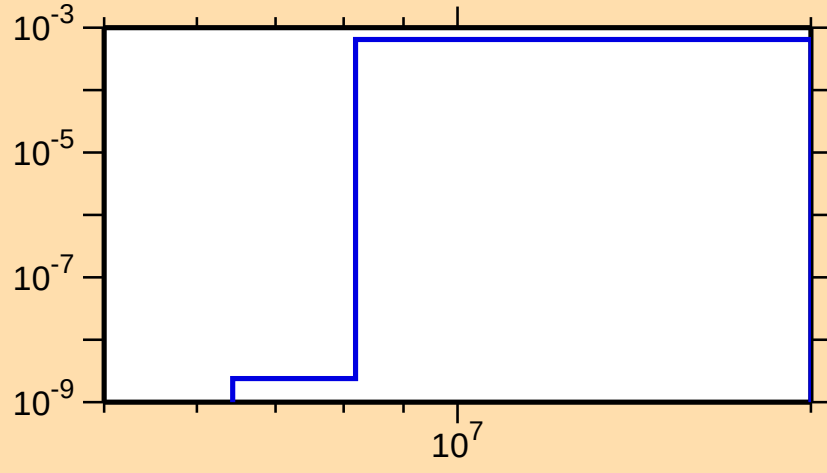
\sigma vs. E for ^{236}\text{Am}(n,d)
