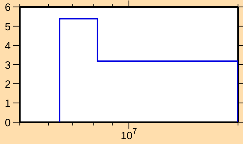
\Delta\sigma/\sigma vs. E for ^{236}\text{Am}(n,\text{tot.})
