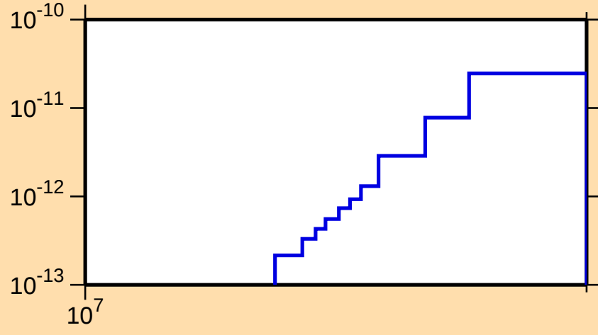
\sigma vs. E for ^{237}\text{Am}(n,p\alpha)
