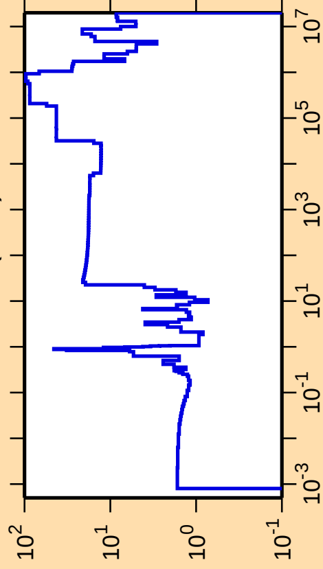
\Delta\sigma/\sigma vs. E for ^{237}\text{Am}(n,\text{el.})
