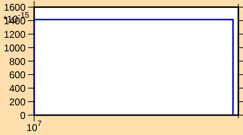
\sigma vs. E for ^{237}\text{Am}(n,p\alpha)
