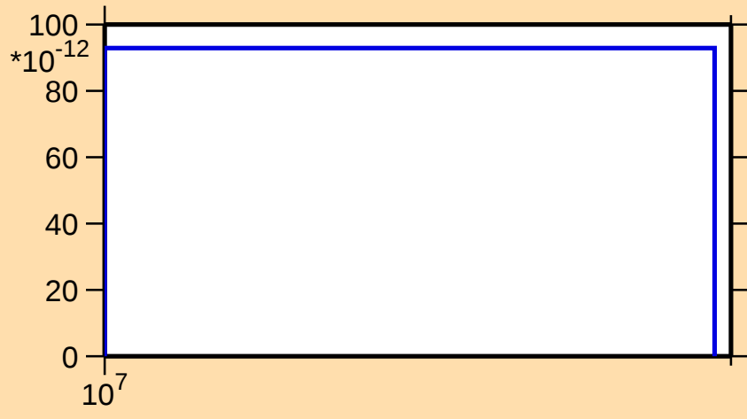
\sigma vs. E for ^{237}\text{Am}(n,\text{He}3)
