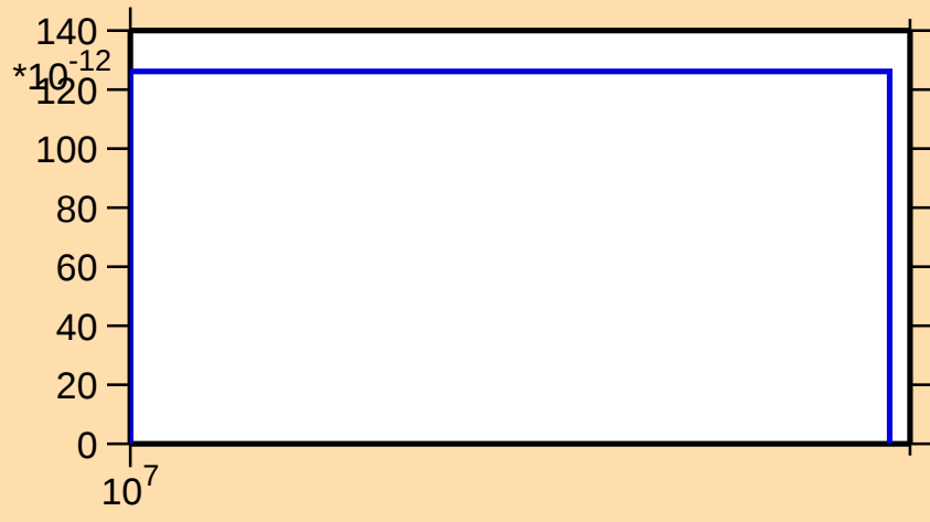
\sigma vs. E for ^{237}\text{Am}(n,2np)
