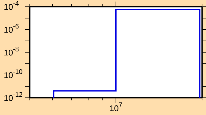
\sigma vs. E for ^{237}\text{Am}(n,t)
