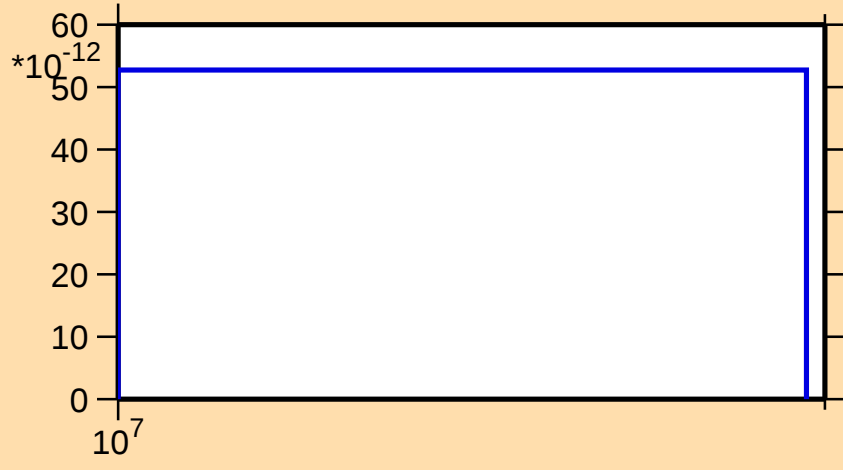
\sigma vs. E for ^{237}\text{Am}(n,\text{nt})
