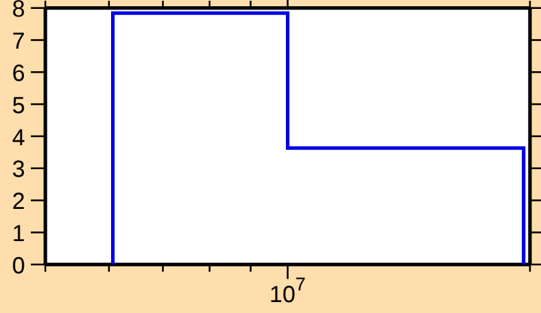
\Delta\sigma/\sigma vs. E for ^{237}\text{Am}(n,\text{tot.})
