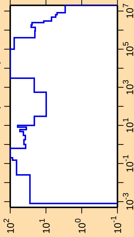
\Delta\sigma/\sigma vs. E for ^{237}\text{Am}(n,\text{nonel.})
