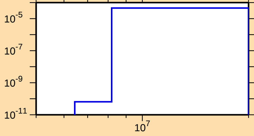
\sigma vs. E for ^{237}\text{Am}(n,np)
