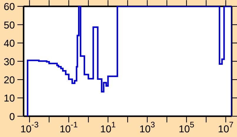
\Delta\sigma/\sigma vs. E for ^{237}\text{Am}(n,\gamma)
