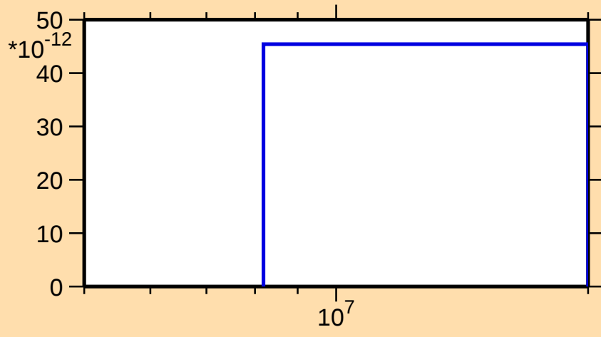
\sigma vs. E for ^{237}\text{Am}(n,nt)
