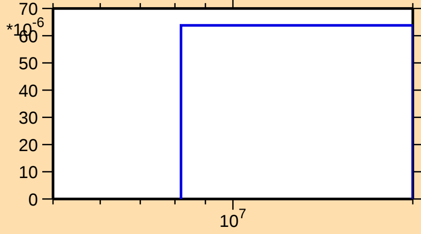
\sigma vs. E for ^{237}\text{Am}(n,3n)
