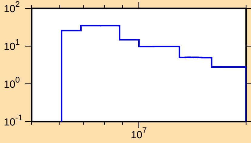
\Delta\sigma/\sigma vs. E for ^{238}\text{Am}(n,\text{el.})
