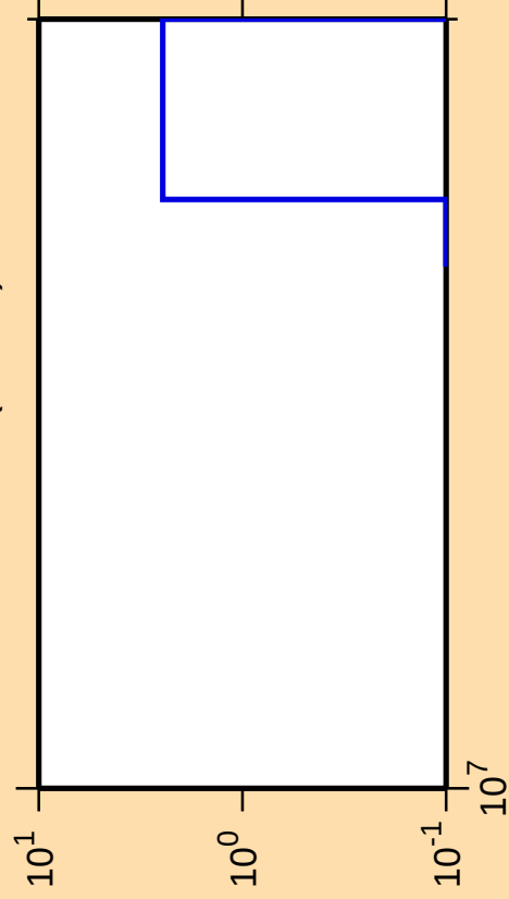
\Delta\sigma/\sigma vs. E for ^{238}\text{Am}(\text{mt } 34)
