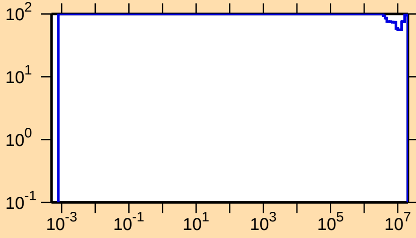
\Delta\sigma/\sigma vs. E for ^{238}\text{Am}(n,p)
