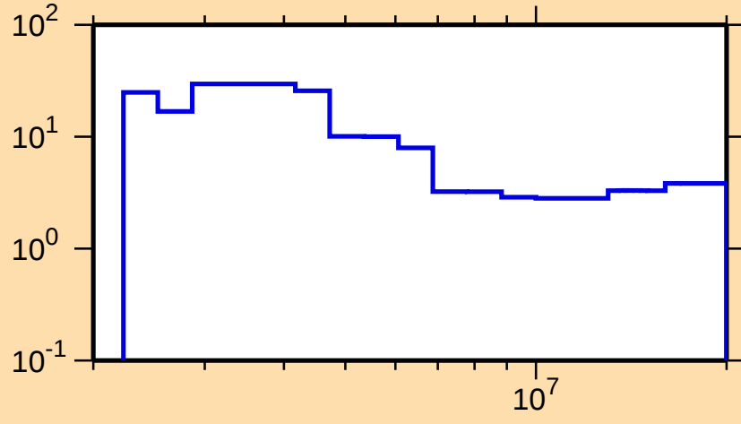
\Delta\sigma/\sigma vs. E for ^{238}\text{Am}(n,f)
