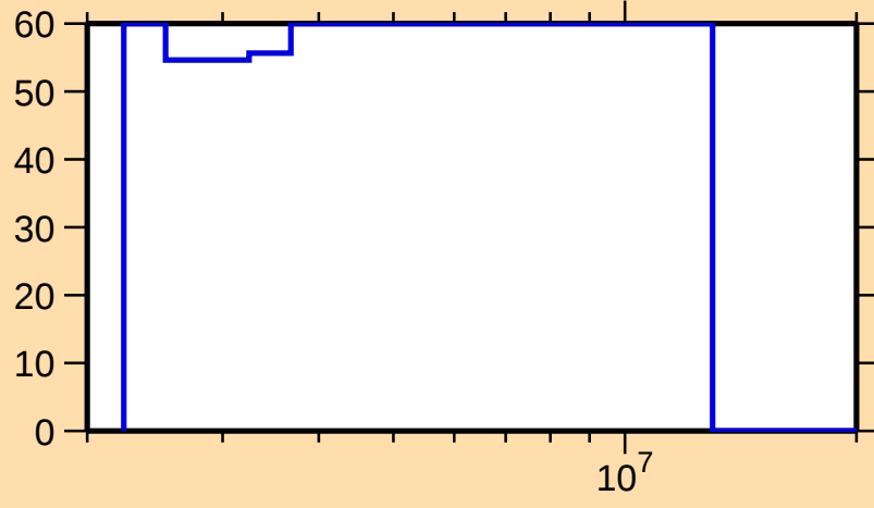
\Delta\sigma/\sigma vs. E for ^{238}\text{Am}(n,n_1)
