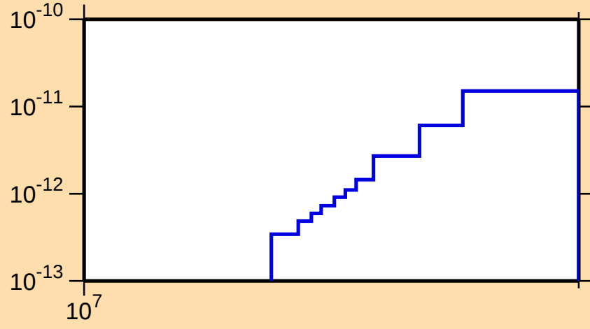
\sigma vs. E for ^{238}\text{Am}(n,p\alpha)
