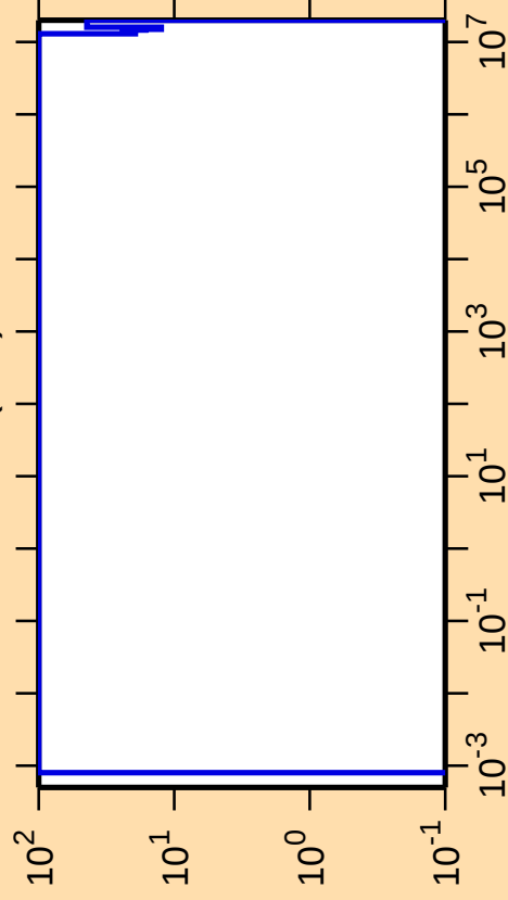
\Delta\sigma/\sigma vs. E for ^{238}\text{Am}(n,\alpha)
