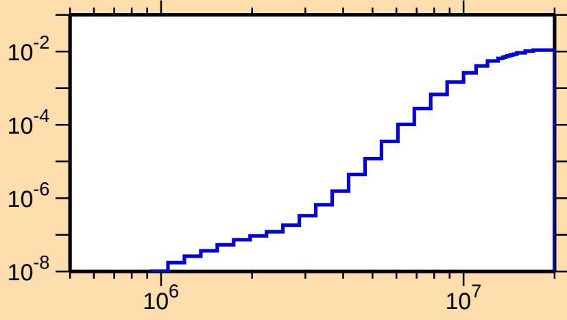
\sigma vs. E for ^{238}\text{Am}(n,p)
