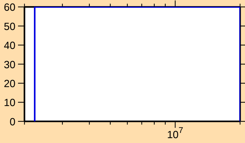
\Delta\sigma/\sigma vs. E for ^{238}\text{Am}(n,\text{inel.})
