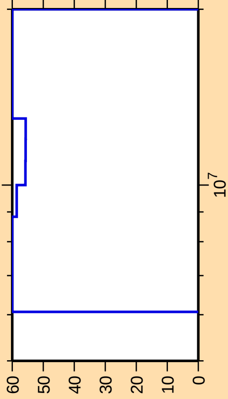
\Delta\sigma/\sigma vs. E for ^{238}\text{Am}(n,p)
