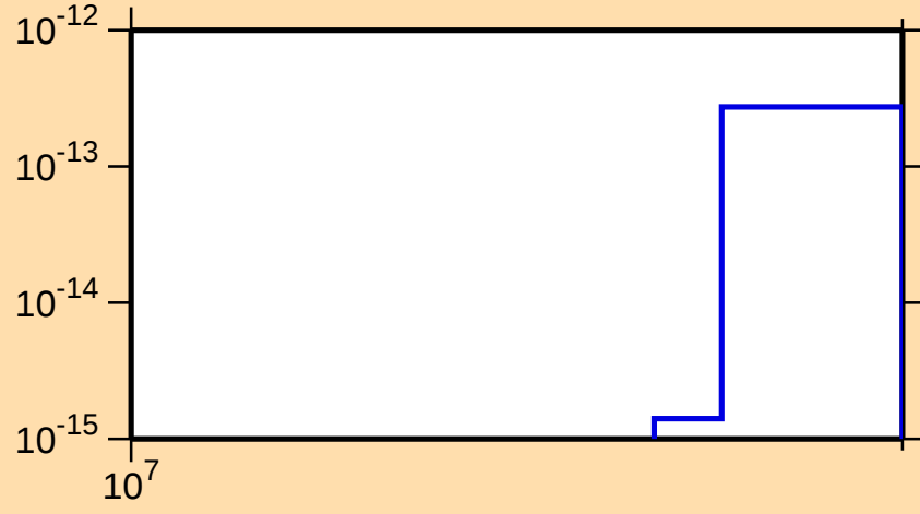
\sigma vs. E for ^{238}\text{Am}(\text{mt } 34)
