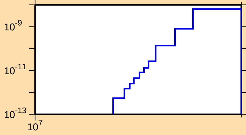
\sigma vs. E for ^{238}\text{Am}(n,\text{He3})
