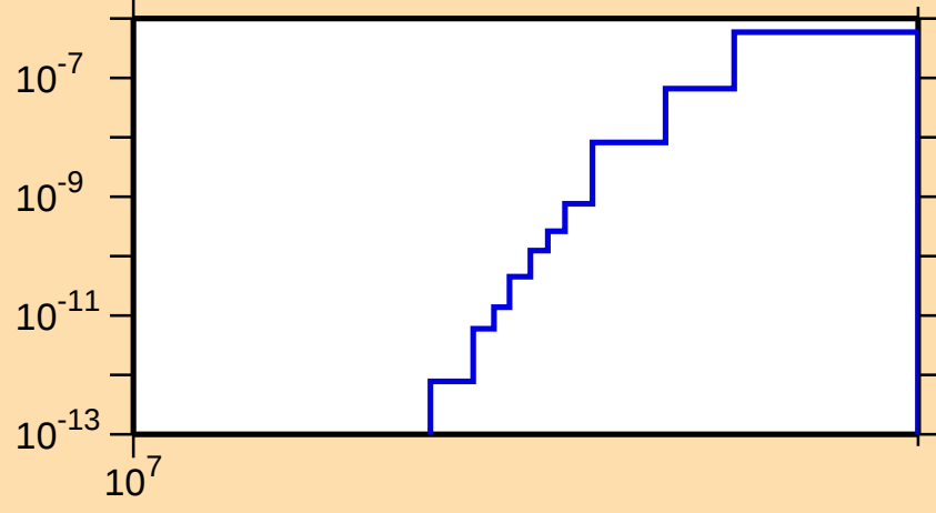
\sigma vs. E for ^{238}\text{Am}(n,2np)
