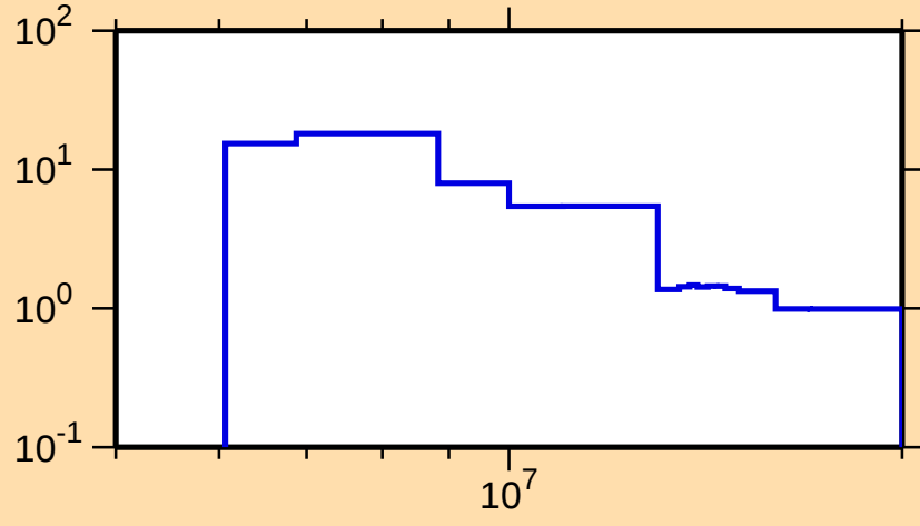
\Delta\sigma/\sigma vs. E for ^{238}\text{Am}(n,\text{tot.})
