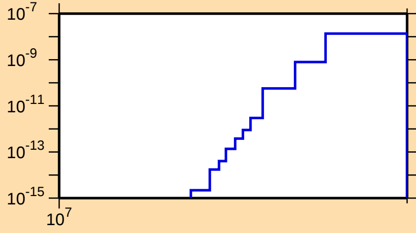
\sigma vs. E for ^{238}\text{Am}(n,nt)
