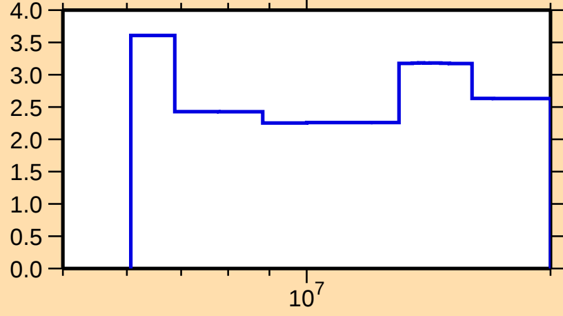
\Delta\sigma/\sigma vs. E for ^{238}\text{Am}(n,\text{nonel.})
