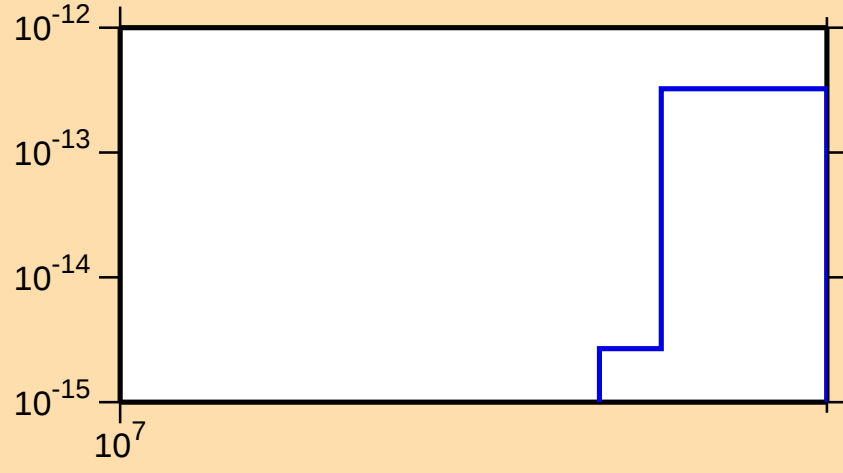
\sigma vs. E for ^{238}\text{Am}(n,3n\alpha)
