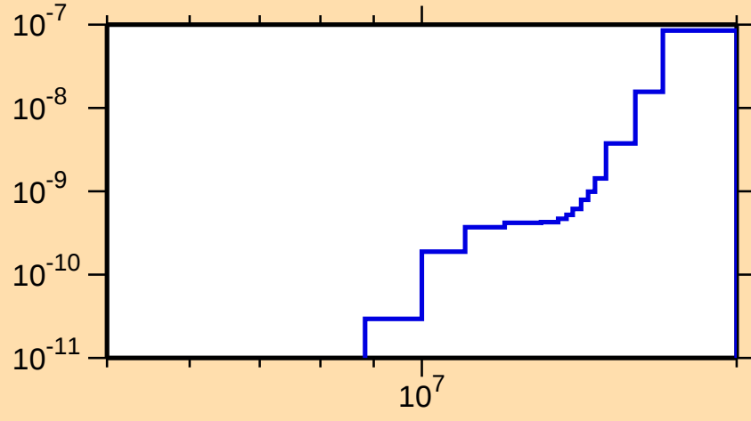
\sigma vs. E for ^{238}\text{Am}(n,2n\alpha)
