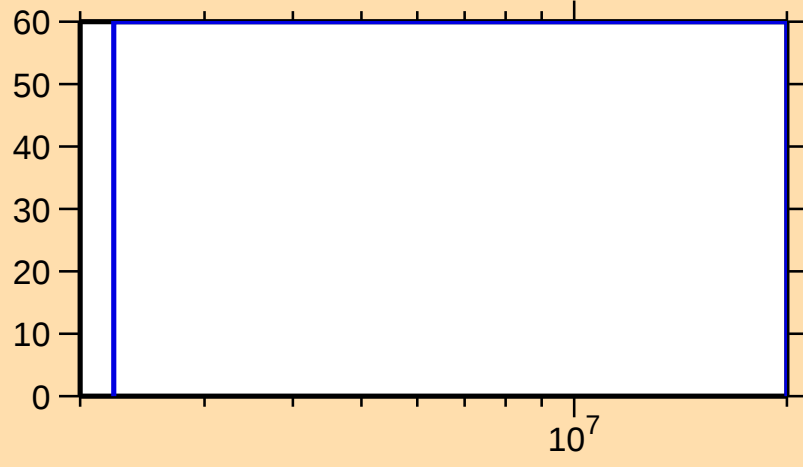
\Delta\sigma/\sigma vs. E for ^{238}\text{Am}(n,\text{inel.})
