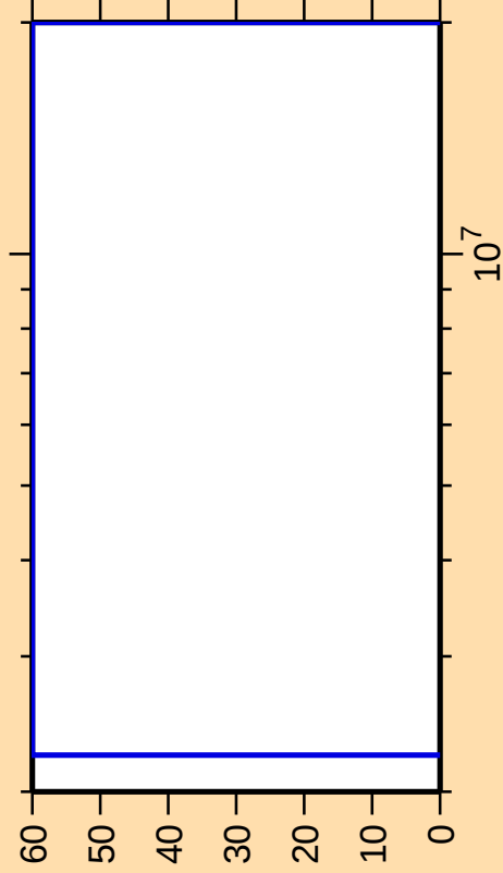
\Delta\sigma/\sigma vs. E for ^{238}\text{Am}(n,n_{\text{cont}})
