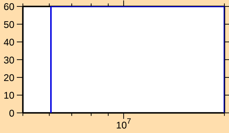
\Delta\sigma/\sigma vs. E for ^{238}\text{Am}(n,2n)
