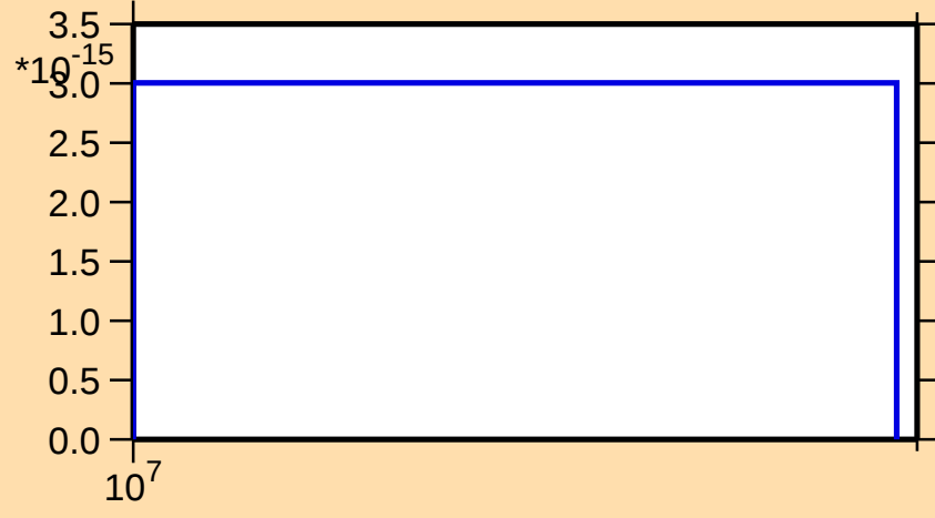
\sigma vs. E for ^{238}\text{Am}(n,3n\alpha)
