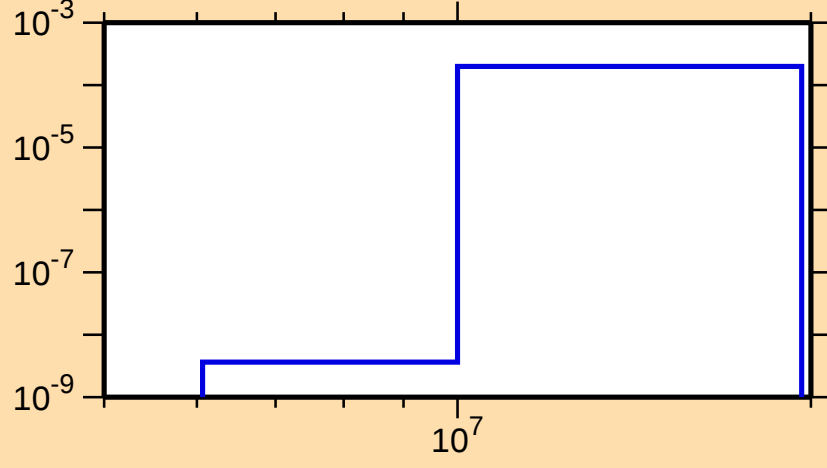
\sigma vs. E for ^{238}\text{Am}(n,np)
