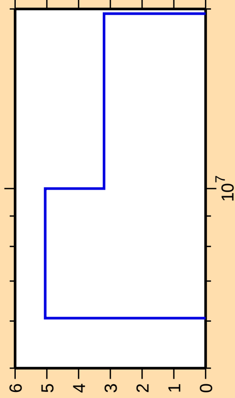
\Delta\sigma/\sigma vs. E for ^{238}\text{Am}(n,f)
