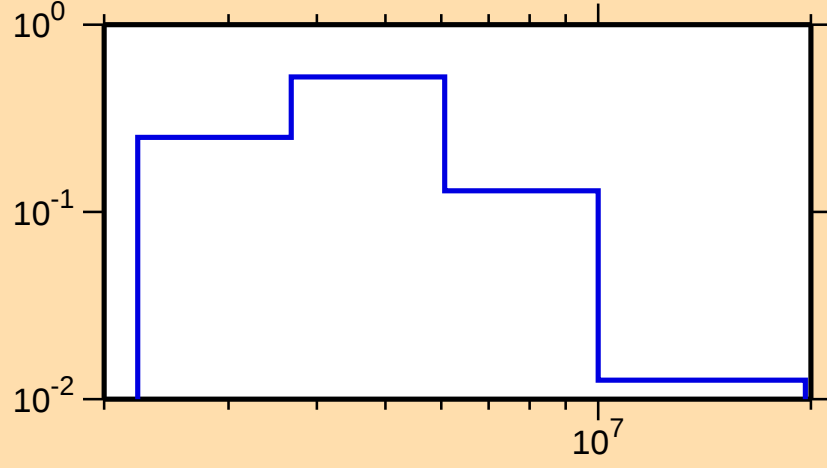
\sigma vs. E for ^{238}\text{Am}(n,n\text{cont.})
