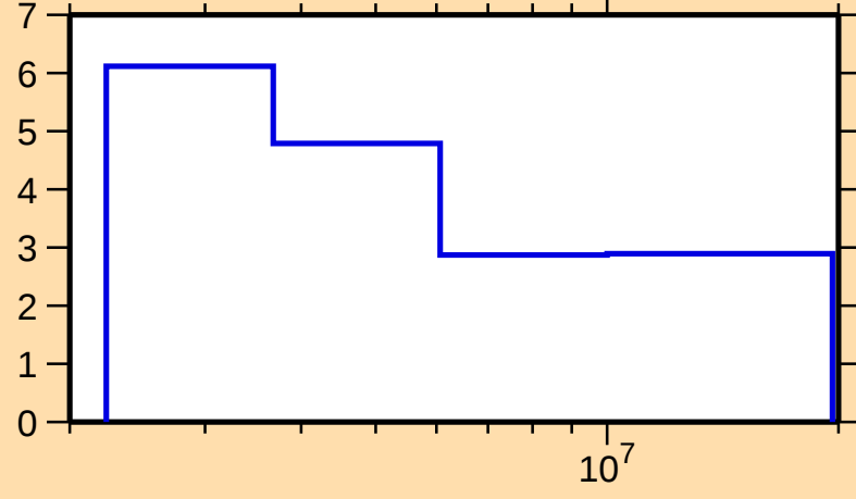
\Delta\sigma/\sigma vs. E for ^{238}\text{Am}(n,\text{nonel.})
