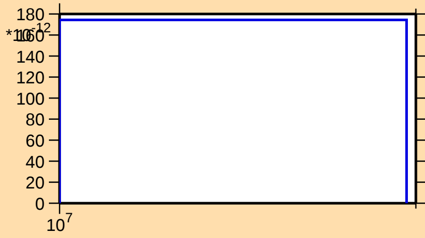
\sigma vs. E for ^{238}\text{Am}(n,\text{nt})
