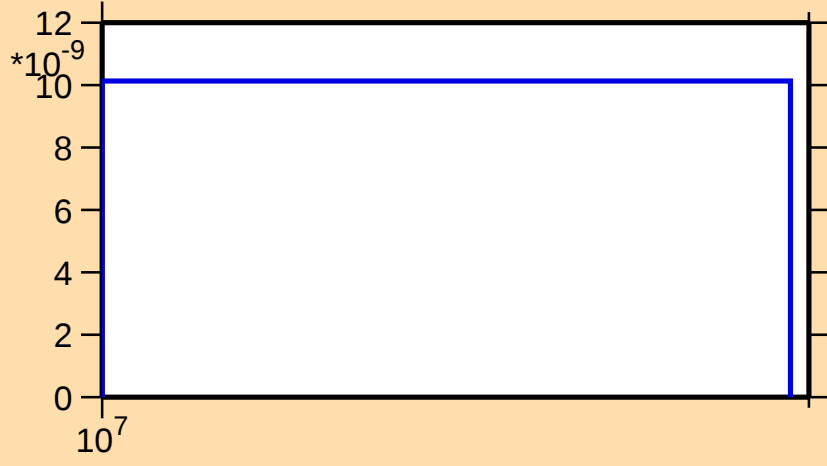
\sigma vs. E for ^{238}\text{Am}(n,2np)
