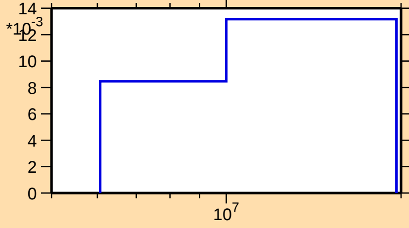
\sigma vs. E for ^{238}\text{Am}(n,2n)
