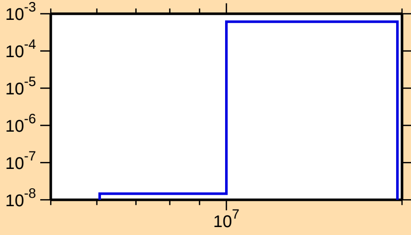
\sigma vs. E for ^{238}\text{Am}(n,d)
