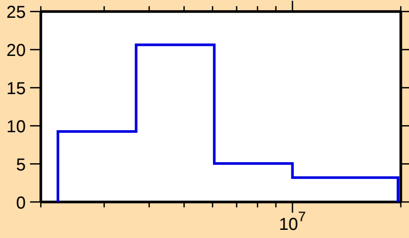
\Delta\sigma/\sigma vs. E for ^{238}\text{Am}(n,f)
