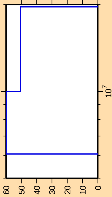
\Delta\sigma/\sigma vs. E for ^{238}\text{Am}(n,d)
