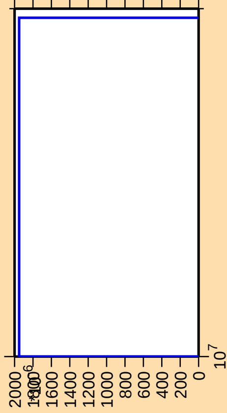
\Delta\sigma/\sigma vs. E for ^{238}\text{Am}(n,3n\alpha)
