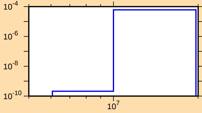
\sigma vs. E for ^{238}\text{Am}(n,t)
