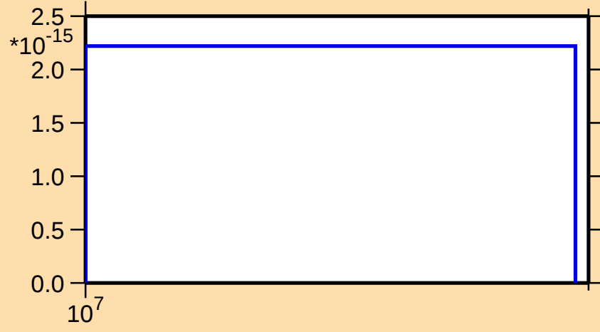
\sigma vs. E for ^{238}\text{Am} (mt 34)
