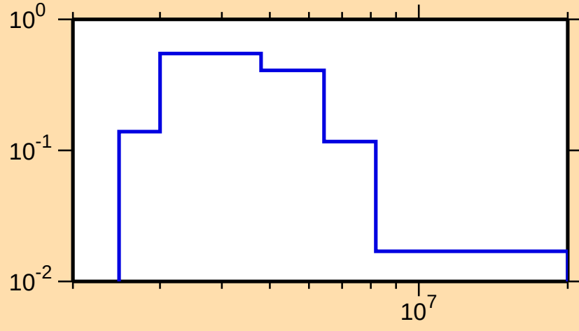
\sigma vs. E for ^{238}\text{Am}(n,\text{inel.})
