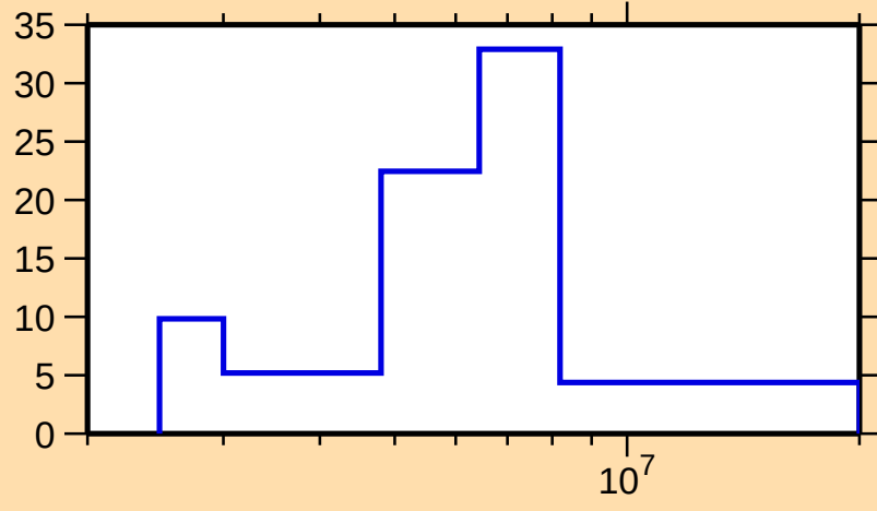
\Delta\sigma/\sigma vs. E for ^{238}\text{Am}(n,\text{el.})
