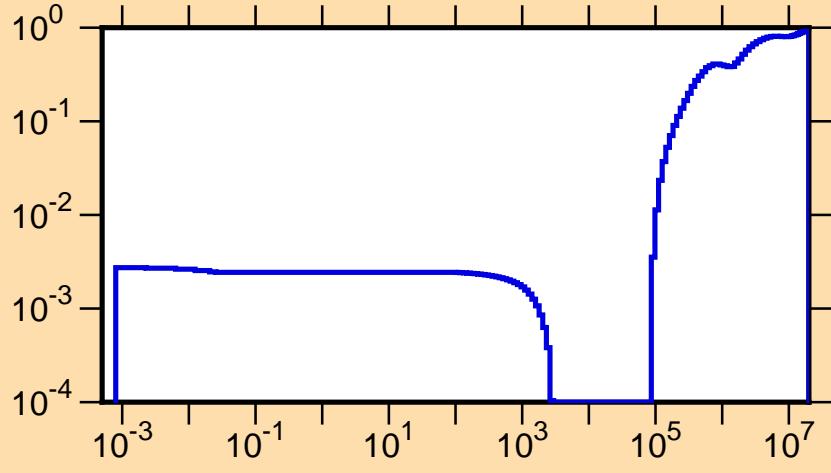
\mu vs. E for ^{244}\text{Am}(\text{mt251})
