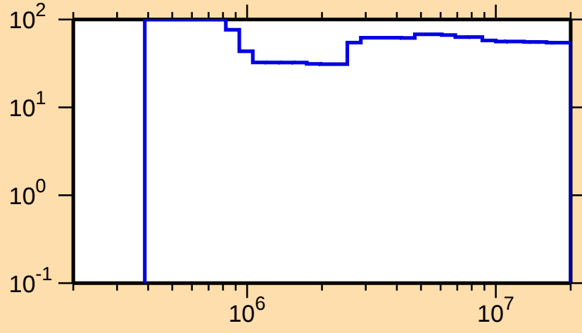
\Delta\sigma/\sigma vs. E for ^{244}\text{Am}(n,n\text{cont.})
