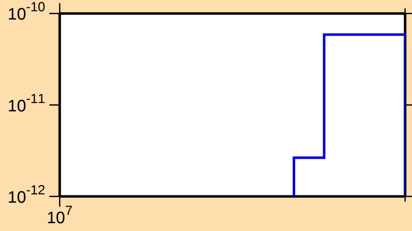
\sigma vs. E for ^{244}\text{Am}(n,\text{He3})
