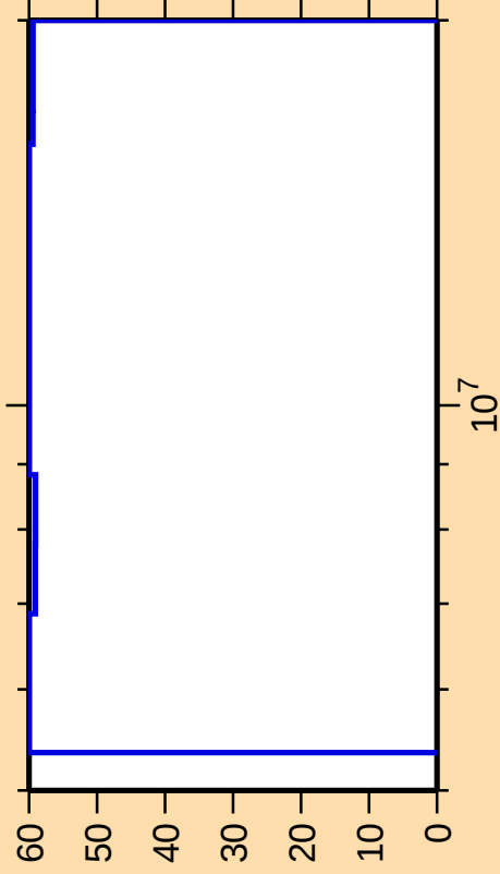
\Delta\sigma/\sigma vs. E for ^{244}\text{Am}(n,2n)
