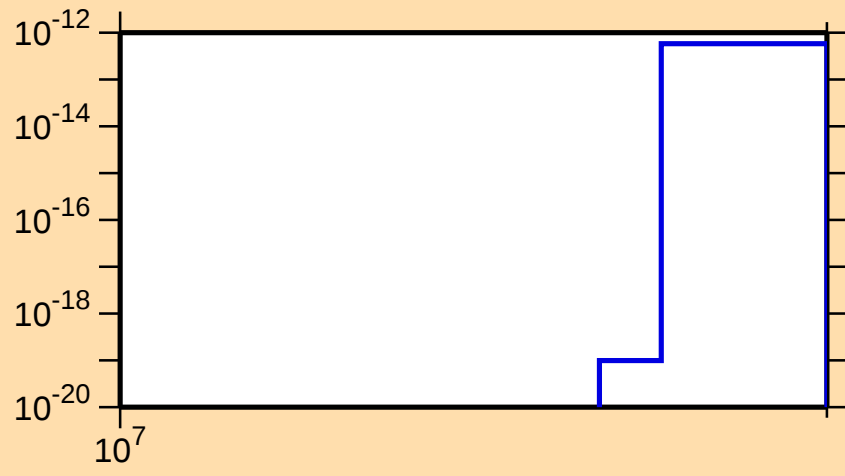
\sigma vs. E for ^{244}\text{Am}(\text{mt } 11)
