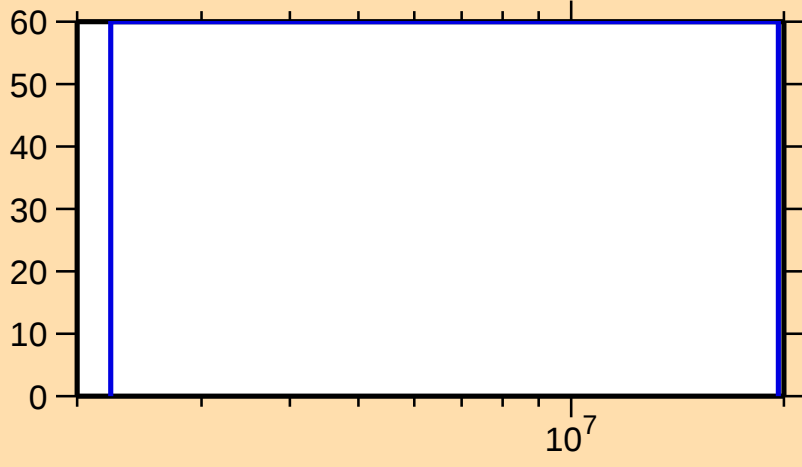
\Delta\sigma/\sigma vs. E for ^{244}\text{Am}(n,p)
