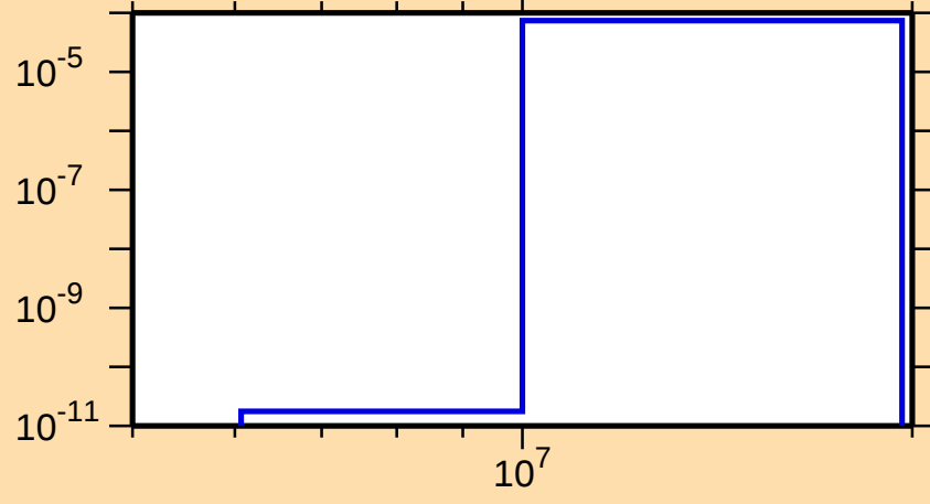
\sigma vs. E for ^{244}\text{Am}(n,np)
