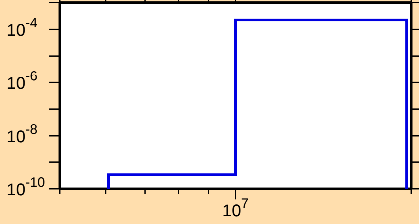
\sigma vs. E for ^{244}\text{Am}(n,d)
