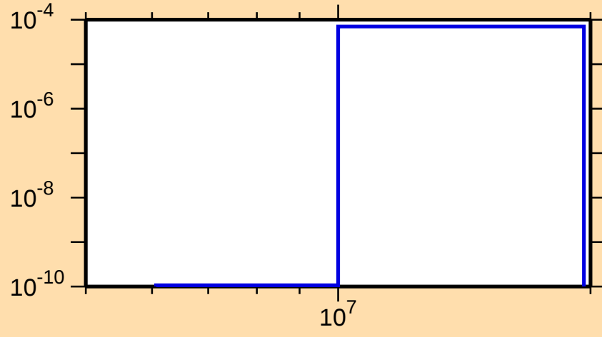
\sigma vs. E for ^{244}\text{Am}(n,t)
