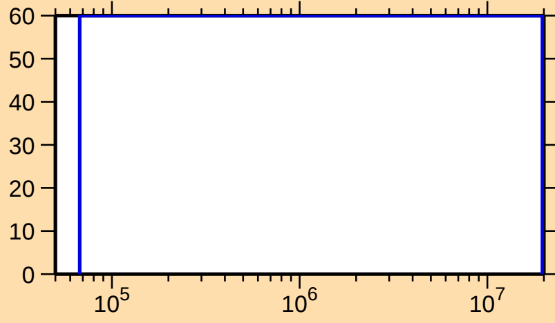
\Delta\sigma/\sigma vs. E for ^{244}\text{Am}(n,f)
