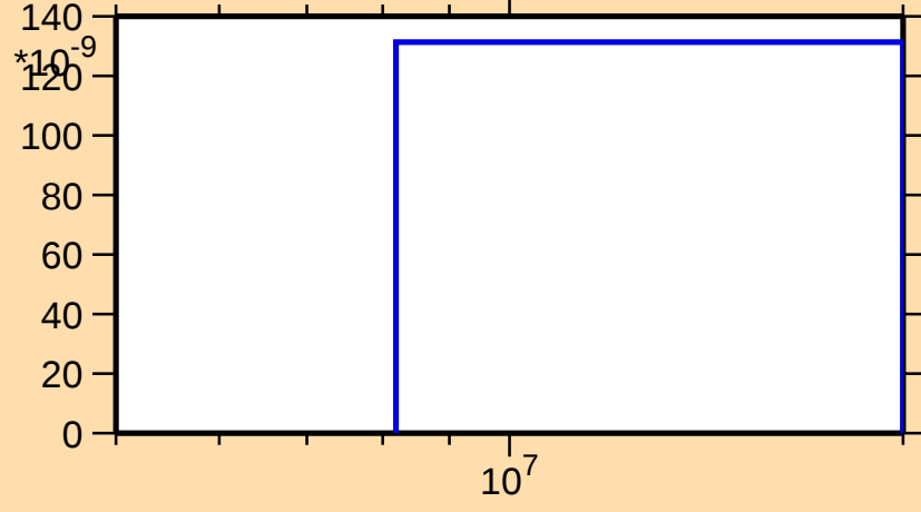
\sigma vs. E for ^{244}\text{Am}(n,\text{nd})
