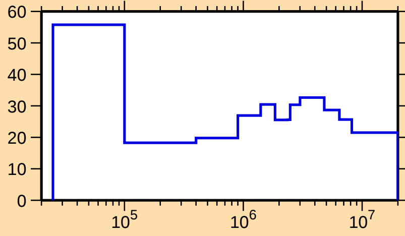
\Delta\sigma/\sigma vs. E for ^{244}\text{Am}(n,\text{nonel.})
