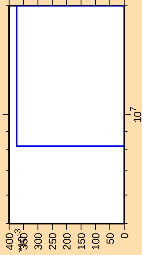
\Delta\sigma/\sigma vs. E for ^{244}\text{Am}(n,3n\alpha)
