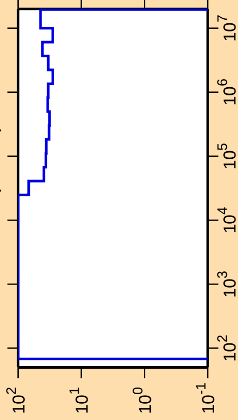
\Delta\sigma/\sigma vs. E for ^{244}\text{Am}(n,\text{inel.})
