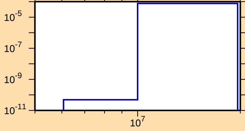
\sigma vs. E for ^{244}\text{Am}(n,t)
