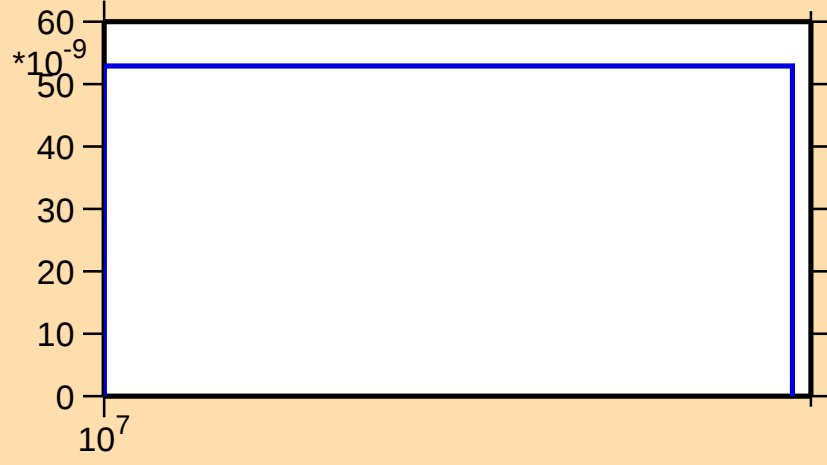
\sigma vs. E for ^{244}\text{Am}(n,2np)
