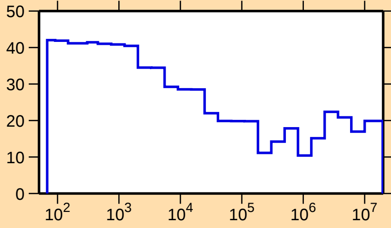
\Delta\sigma/\sigma vs. E for ^{244}\text{Am}(n,\text{tot.})
