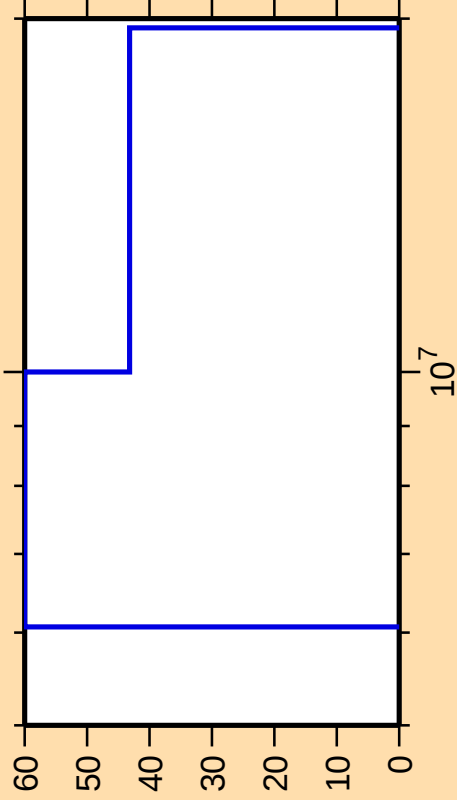
\Delta\sigma/\sigma vs. E for ^{244}\text{Am}(n,d)
