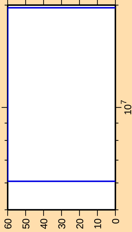
\Delta\sigma/\sigma vs. E for ^{244}\text{Am}(n,t)
