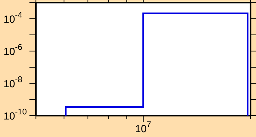
\sigma vs. E for ^{244}\text{Am}(n,d)
