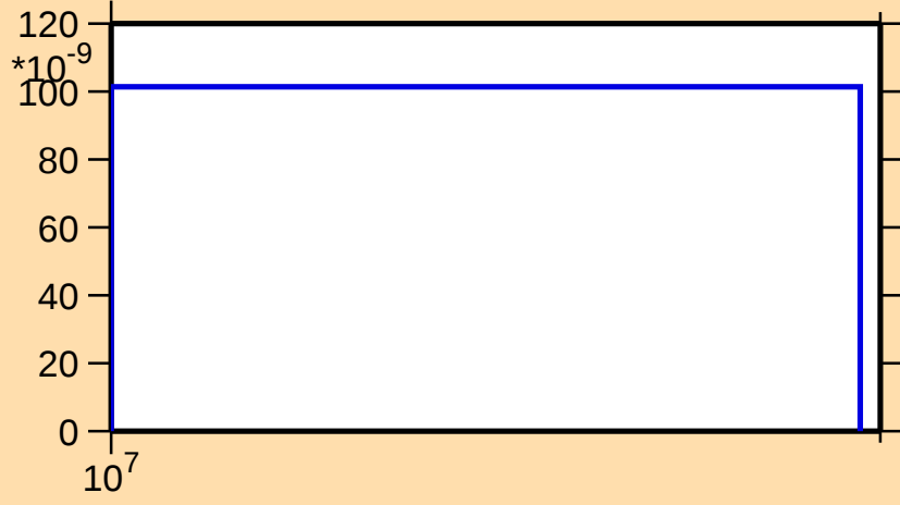
\sigma vs. E for ^{244}\text{Am}(n,\text{nt})
