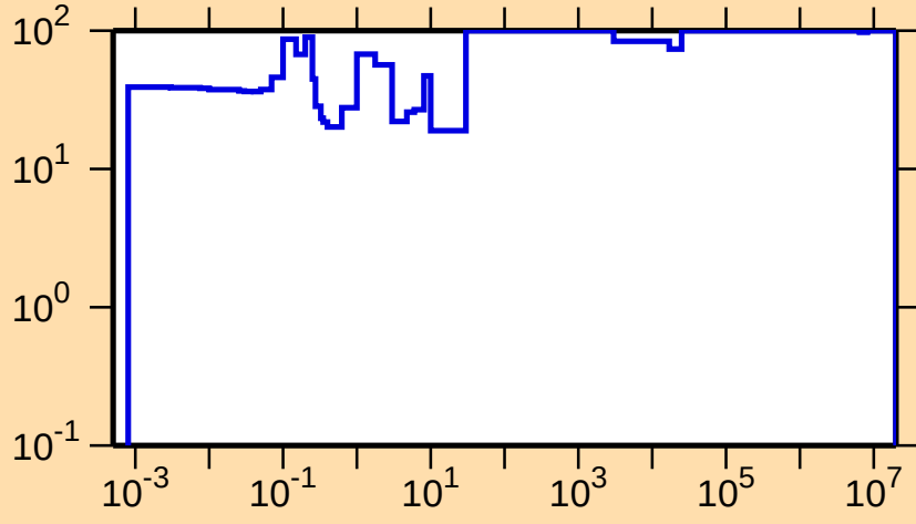
\Delta\sigma/\sigma vs. E for ^{244}\text{Am}(n,\gamma)
