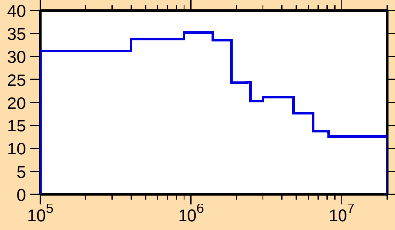
\Delta\sigma/\sigma vs. E for ^{244}\text{Am}(n,n\text{onel.})
