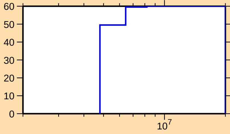
\Delta\sigma/\sigma vs. E for ^{244}\text{Am}(n,2n)
