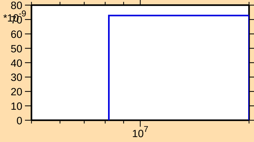
\sigma vs. E for ^{244}\text{Am}(n,2n\alpha)
