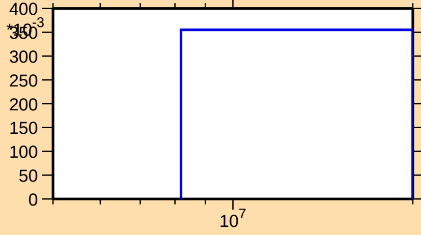
\sigma vs. E for ^{244}\text{Am}(n,3n)
