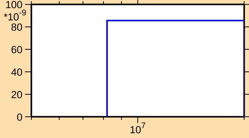
\sigma vs. E for ^{244}\text{Am}(n,nt)
