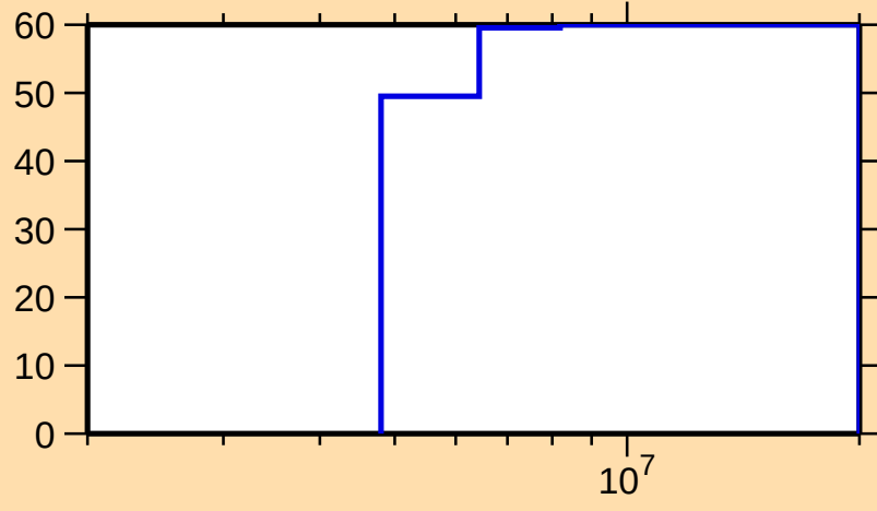
\Delta\sigma/\sigma vs. E for ^{244}\text{Am}(n,2n)
