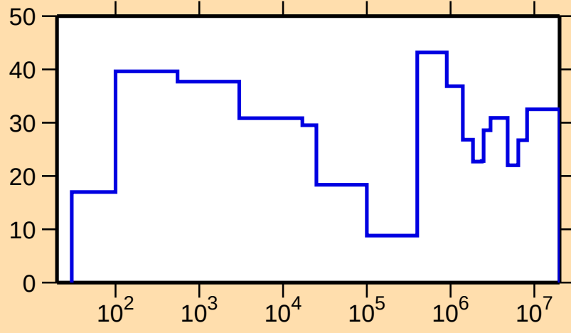
\Delta\sigma/\sigma vs. E for ^{244}\text{Am}(n,\text{el.})
