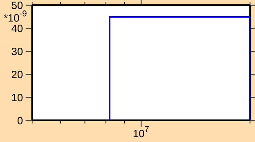
\sigma vs. E for ^{244}\text{Am}(n,2np)
