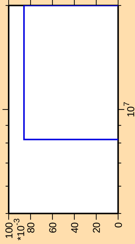
\Delta\sigma/\sigma vs. E for ^{244}\text{Am}(\text{mt } 11)
