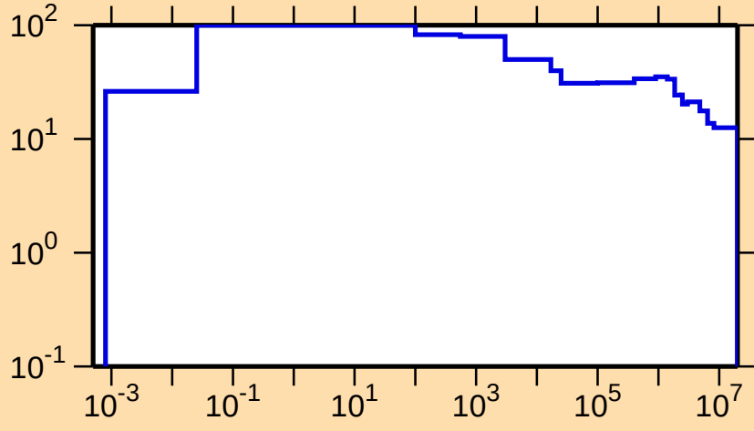
\Delta\sigma/\sigma vs. E for ^{244}\text{Am}(n,\text{nonel.})
