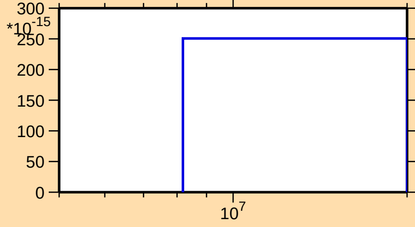
\sigma vs. E for ^{244}\text{Am}(n,3n\alpha)
