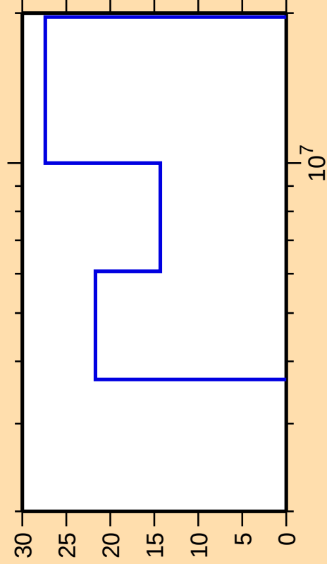
\Delta\sigma/\sigma vs. E for ^{39}\text{Ar}(n,\text{ncont.})
