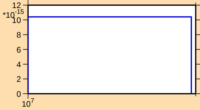
\sigma vs. E for ^{39}\text{Ar}(n,\text{nt})
