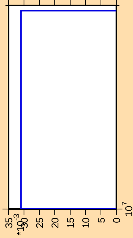
\Delta\sigma/\sigma vs. E for ^{39}\text{Ar}(n,\text{nt})
