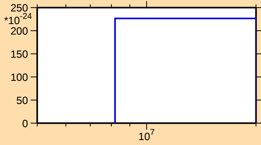
\sigma vs. E for ^{39}\text{Ar}(\text{mt } 45)
