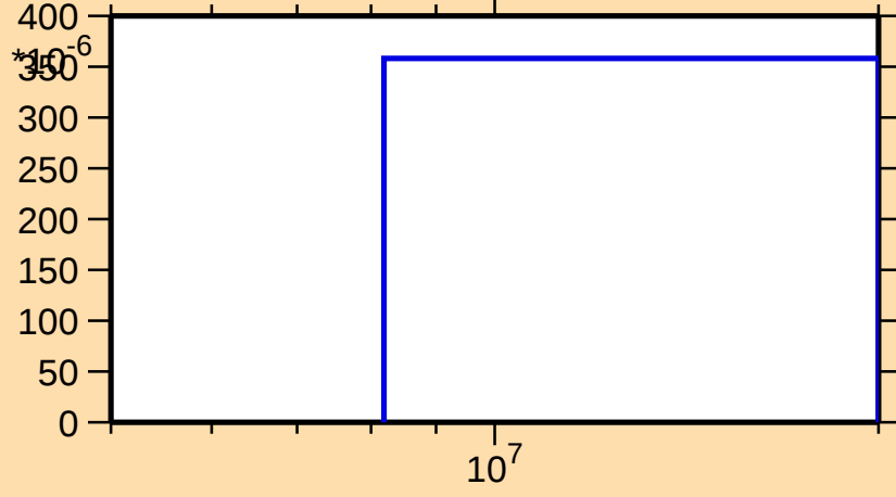
\sigma vs. E for ^{39}\text{Ar}(n,t)
