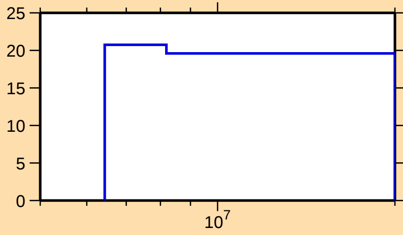
\Delta\sigma/\sigma vs. E for ^{39}\text{Ar}(n,2n)
