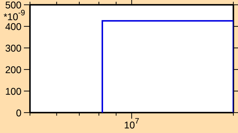
\sigma vs. E for ^{39}\text{Ar}(n,2np)
