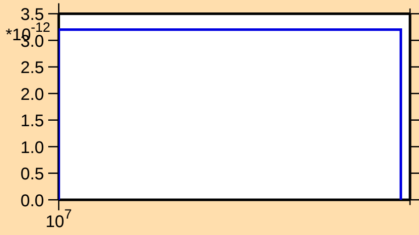
\sigma vs. E for ^{41}\text{Ar}(n,nt)
