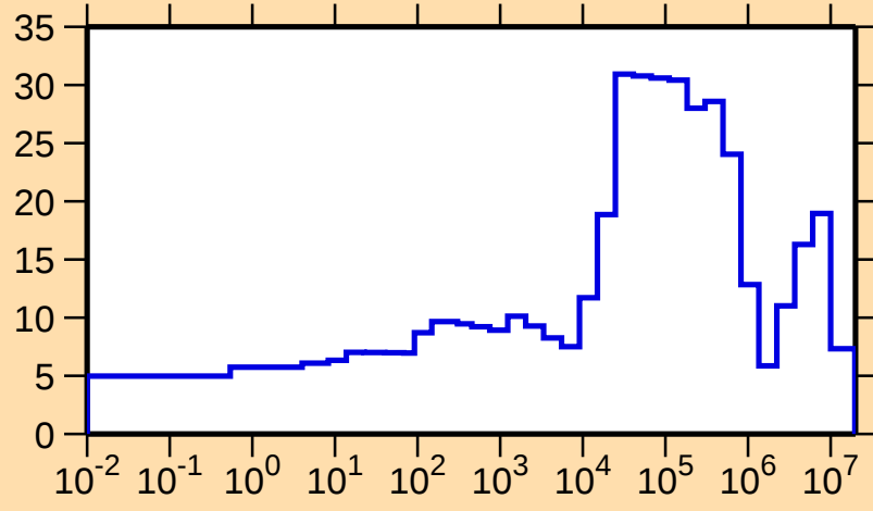
\Delta\sigma/\sigma vs. E for ^{41}\text{Ar}(n,\text{el.})
