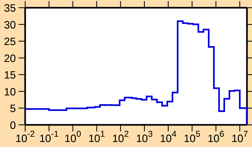
\Delta\sigma/\sigma vs. E for ^{41}\text{Ar}(n,\text{tot.})
