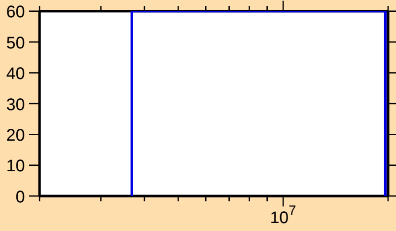
\Delta\sigma/\sigma vs. E for ^{41}\text{Ar}(n,\gamma)
