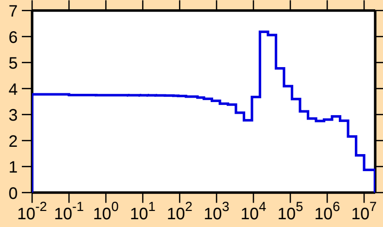
\sigma vs. E for ^{41}\text{Ar}(n,\text{el.})
