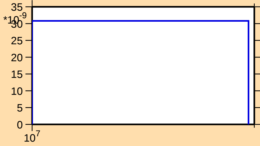
\sigma vs. E for ^{41}\text{Ar}(n,\text{nd})
