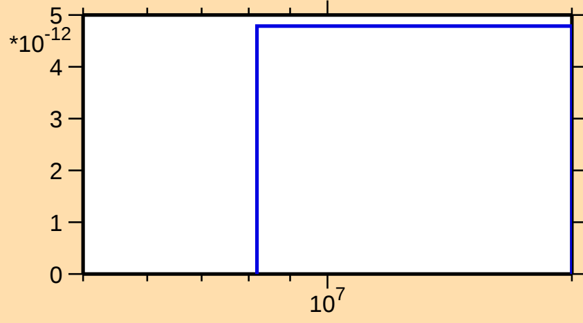
\sigma vs. E for ^{41}\text{Ar}(n,\text{nt})
