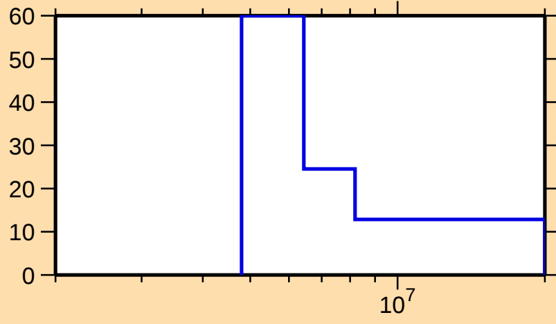
\Delta\sigma/\sigma vs. E for ^{41}\text{Ar}(n,2n)
