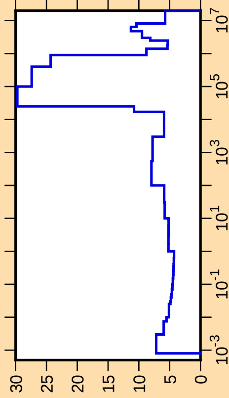
\Delta\sigma/\sigma vs. E for ^{41}\text{Ar}(n,\text{tot.})
