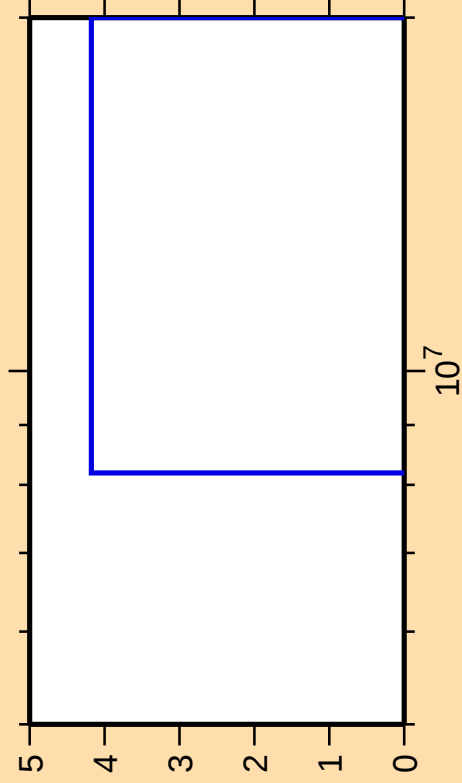
\Delta\sigma/\sigma vs. E for ^{41}\text{Ar}(n,\text{nt})
