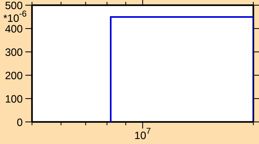
\sigma vs. E for ^{41}\text{Ar}(n,d)
