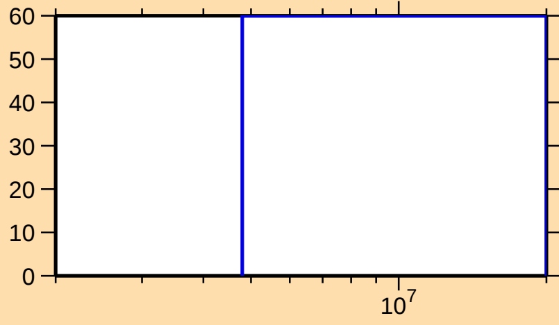
\Delta\sigma/\sigma vs. E for ^{41}\text{Ar}(n,p)
