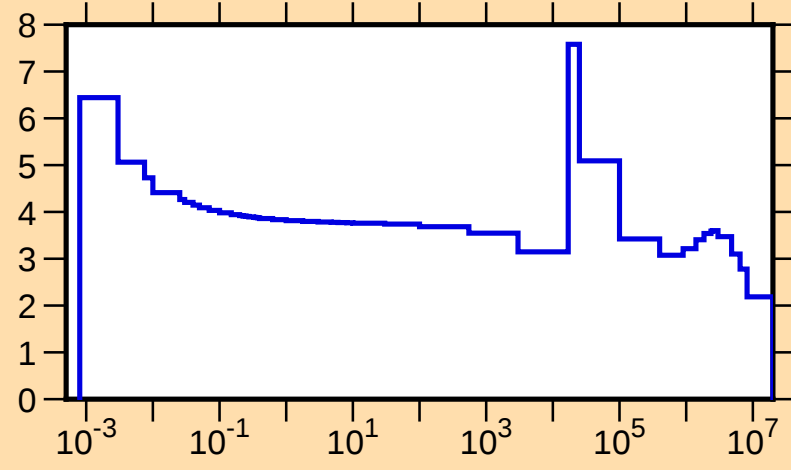
\sigma vs. E for ^{41}\text{Ar}(n,\text{tot.})
