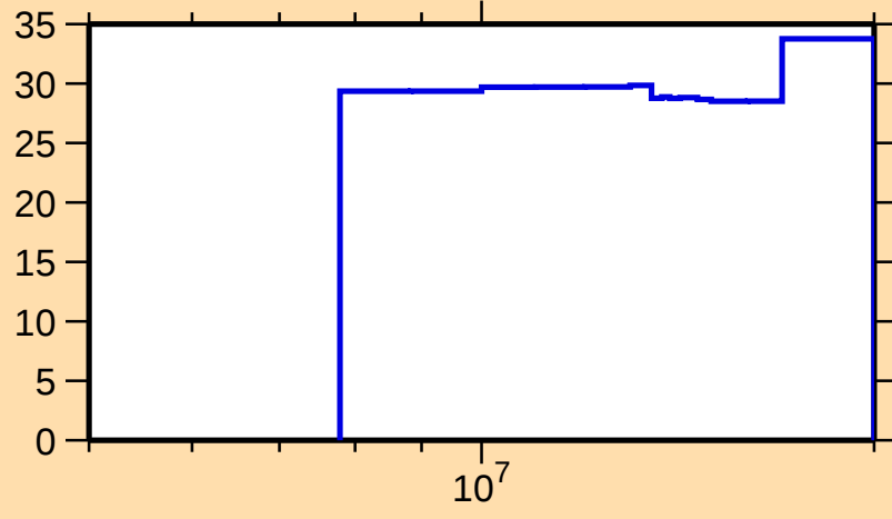
\Delta\sigma/\sigma vs. E for ^{46}\text{Ar}(n,\text{tot.})
