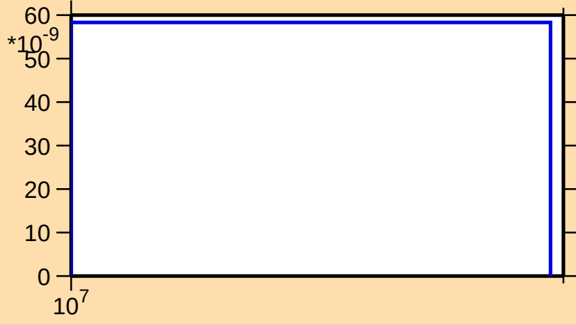
\sigma vs. E for ^{46}\text{Ar}(n,\alpha)
