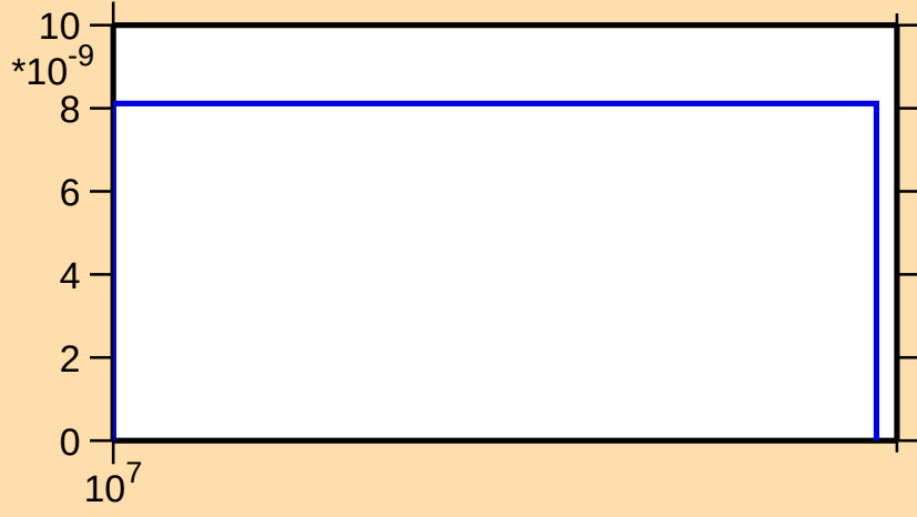
\sigma vs. E for ^{46}\text{Ar}(n,d)
