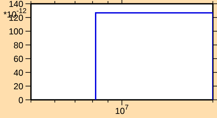
\sigma vs. E for ^{46}\text{Ar}(n,n\alpha)
