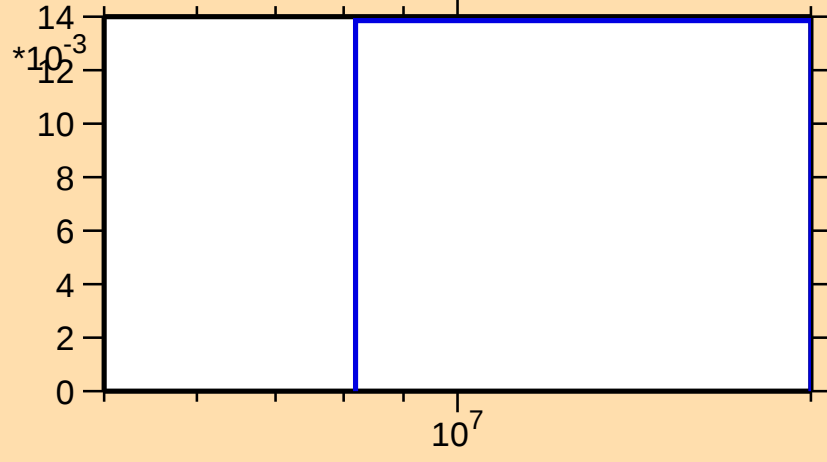
\sigma vs. E for ^{46}\text{Ar}(n,3n)
