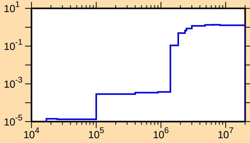
\sigma vs. E for ^{46}\text{Ar}(n,\text{nonel.})
