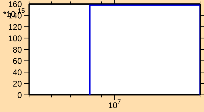
\sigma vs. E for ^{46}\text{Ar}(n,np)
