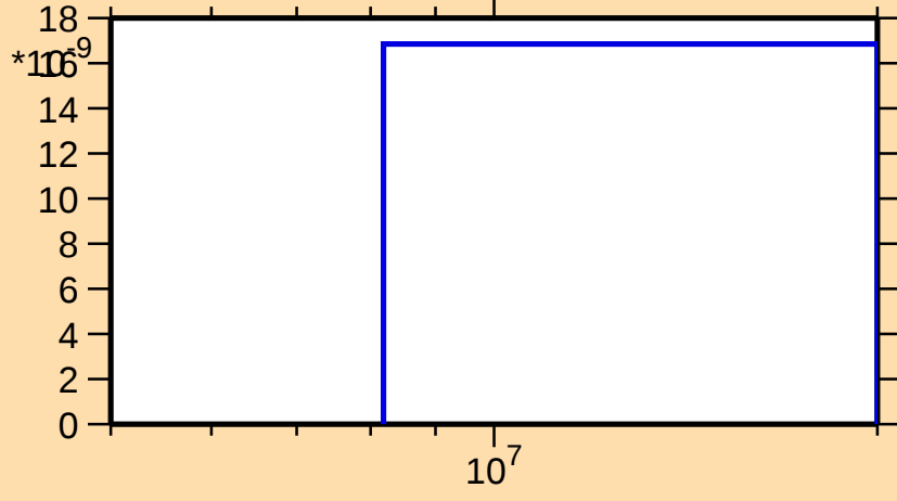
\sigma vs. E for ^{46}\text{Ar}(n,p)
