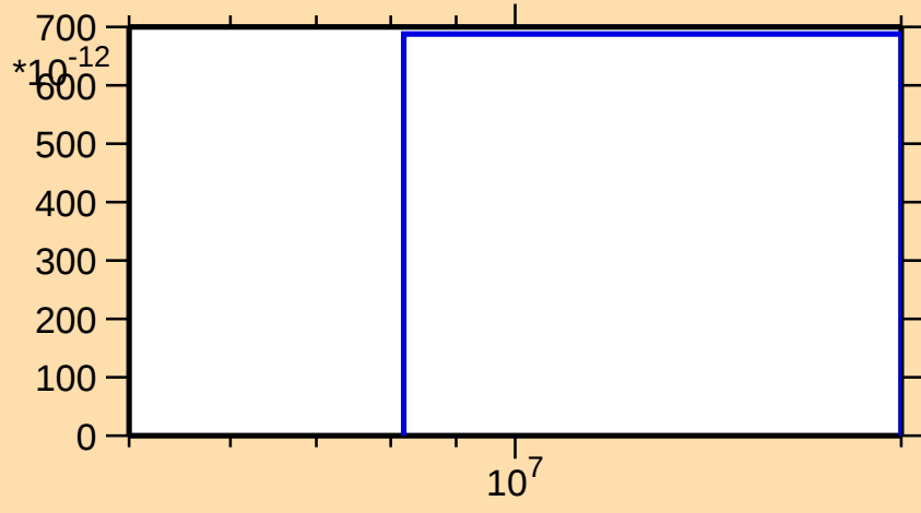
\sigma vs. E for ^{46}\text{Ar}(n,t)
