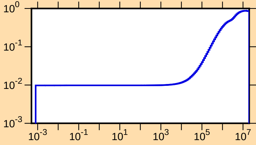
\mu vs. E for ^{69}\text{As}(\text{mt251})
