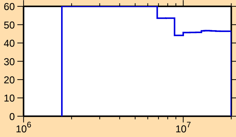
\Delta\sigma/\sigma vs. E for ^{69}\text{As}(n,n\text{cont.})
