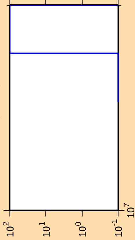
\Delta\sigma/\sigma vs. E for ^{69}\text{As}(\text{mt } 34)
