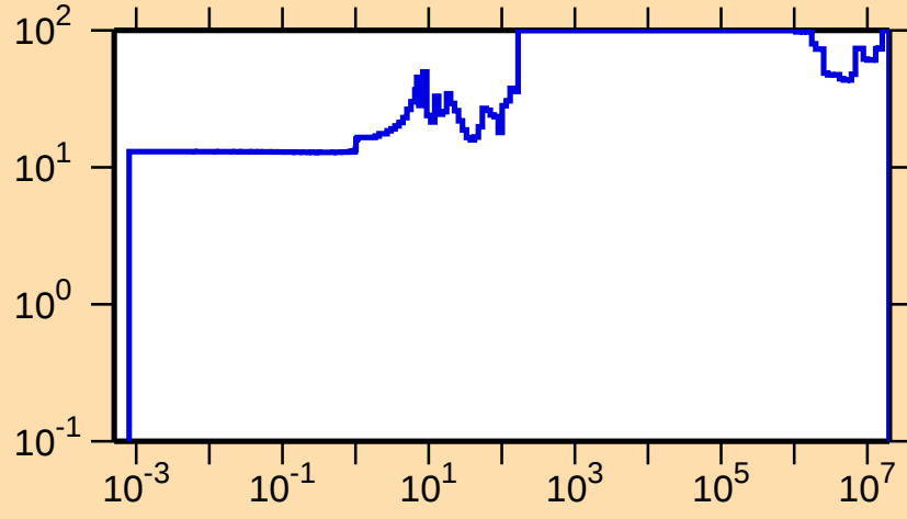
\Delta\sigma/\sigma vs. E for ^{69}\text{As}(n,\gamma)
