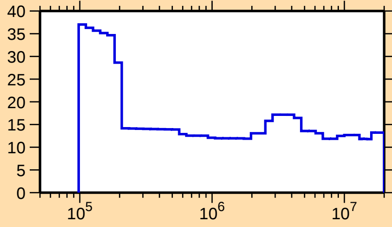
\Delta\sigma/\sigma vs. E for ^{69}\text{As}(n,\text{nonel.})
