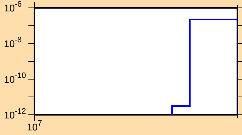
\sigma vs. E for ^{69}\text{As}(n,\text{pt})
