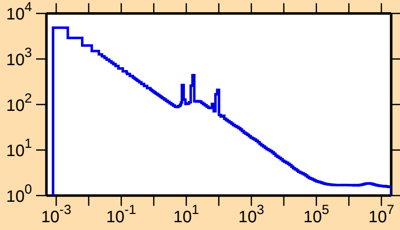
\sigma vs. E for ^{69}\text{As}(n,\text{nonel.})
