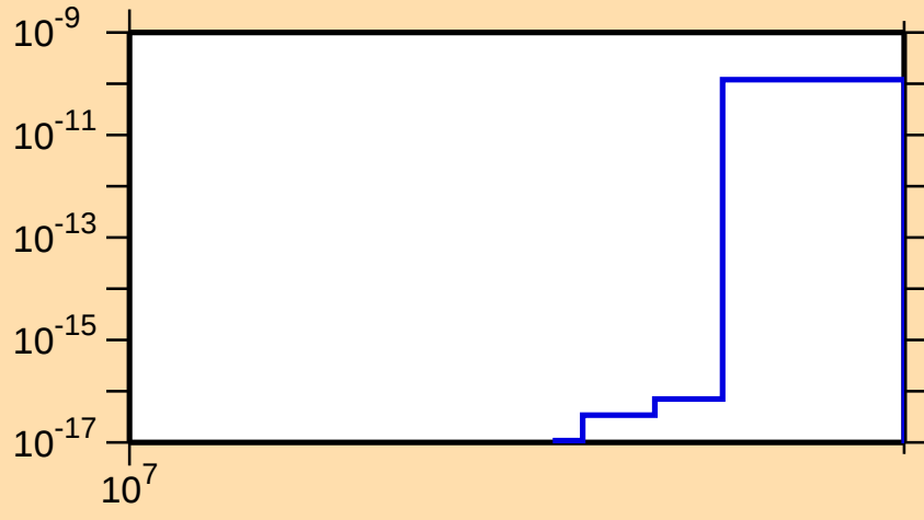
\sigma vs. E for ^{69}\text{As}(\text{mt } 34)
