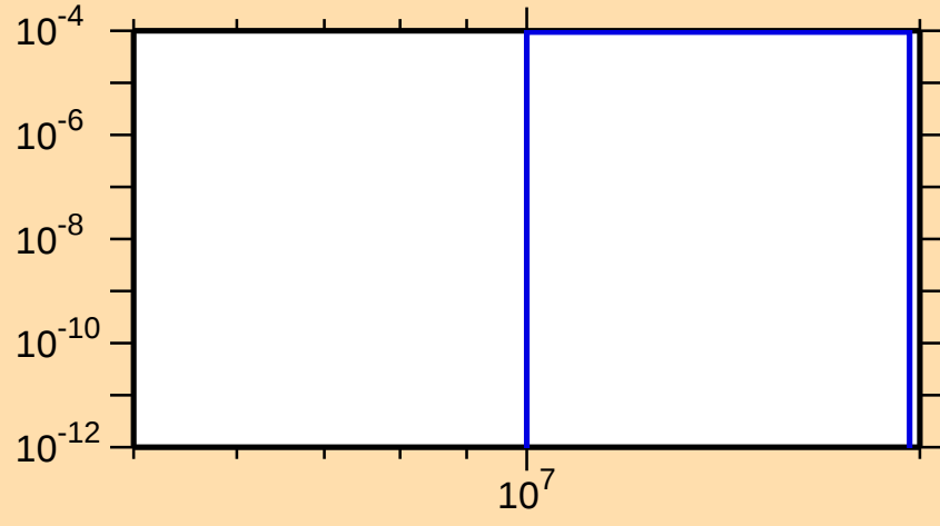
\sigma vs. E for ^{69}\text{As}(n,\text{pd})
