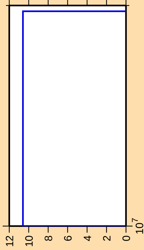
\Delta\sigma/\sigma vs. E for ^{69}\text{As}(n,nt)
