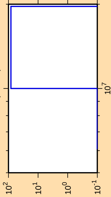
\Delta\sigma/\sigma vs. E for ^{69}\text{As}(\text{mt } 45)
