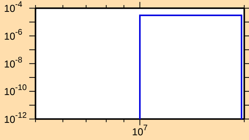
\sigma vs. E for ^{69}\text{As}(\text{mt } 45)
