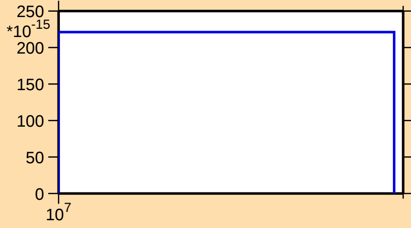
\sigma vs. E for ^{69}\text{As}(n,2n\alpha)
