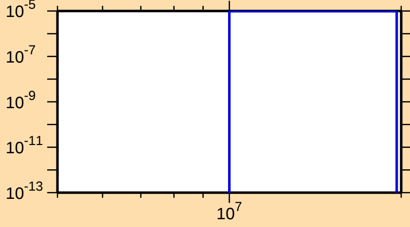
\sigma vs. E for ^{69}\text{As}(\text{mt117})
