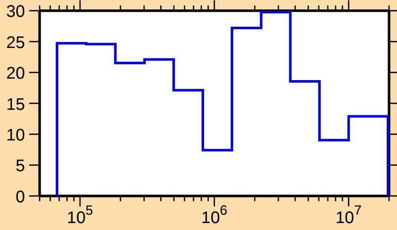
\Delta\sigma/\sigma vs. E for ^{69}\text{As}(n,\text{el.})
