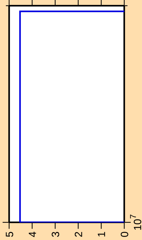
\Delta\sigma/\sigma vs. E for ^{69}\text{As}(\text{mt } 34)
