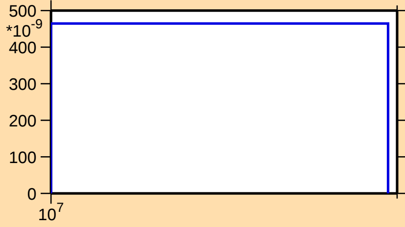
\sigma vs. E for ^{69}\text{As}(n,2np)
