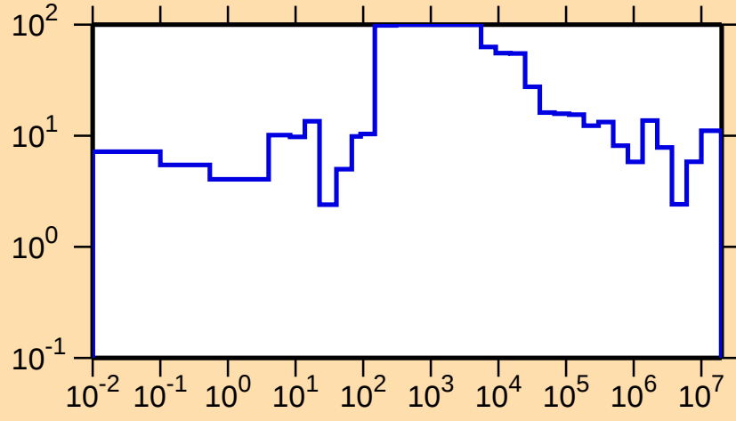
\Delta\sigma/\sigma vs. E for ^{69}\text{As}(n,\text{tot.})
