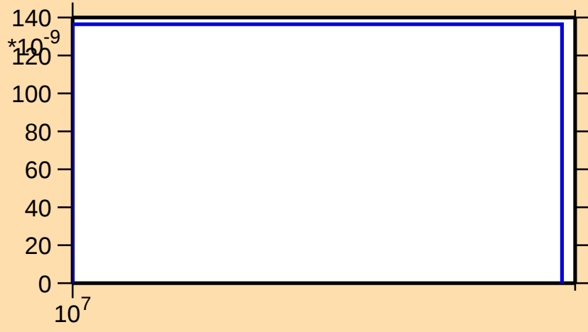
\sigma vs. E for ^{69}\text{As}(n,\text{nd})
