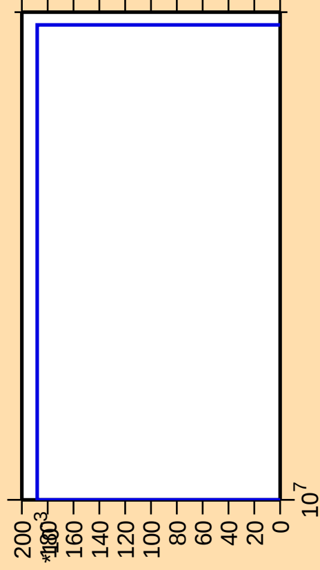
\Delta\sigma/\sigma vs. E for ^{69}\text{As}(n,2n\alpha)
