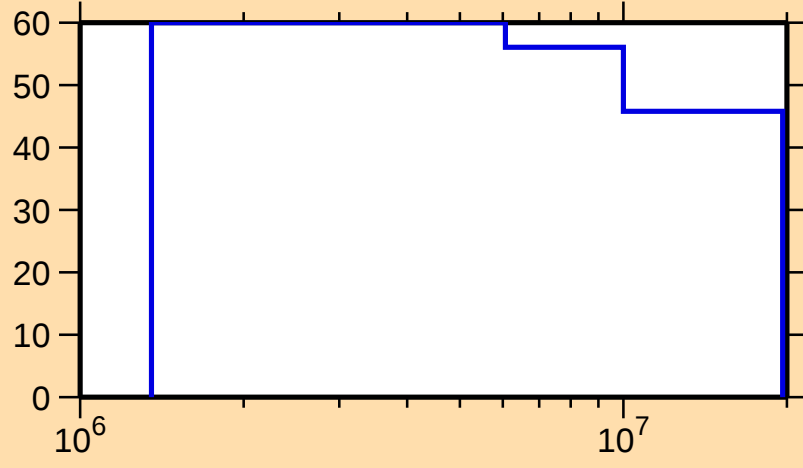
\Delta\sigma/\sigma vs. E for ^{69}\text{As}(n,n\text{cont.})
