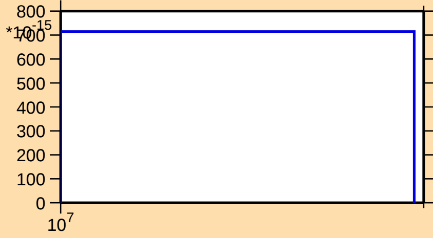
\sigma vs. E for ^{69}\text{As}(\text{mt } 34)
