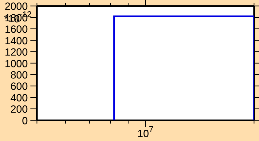
\sigma vs. E for ^{69}\text{As}(n,\text{pt})
