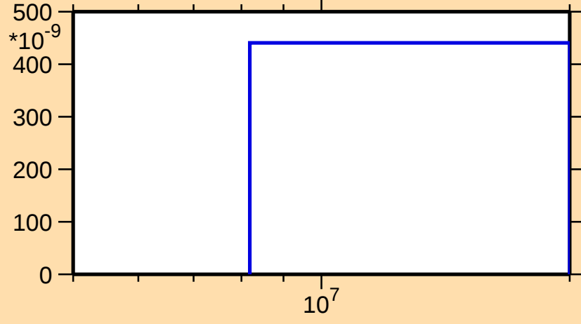
\sigma vs. E for ^{69}\text{As}(n,2np)
