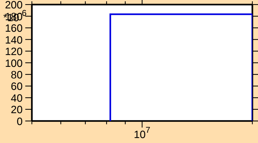
\sigma vs. E for ^{69}\text{As}(n,t)
