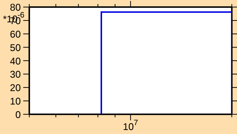
\sigma vs. E for ^{69}\text{As}(n,\text{pd})
