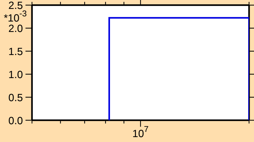
\sigma vs. E for ^{69}\text{As}(n,2n)
