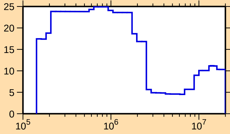
\Delta\sigma/\sigma vs. E for ^{71}\text{As}(n,\text{tot.})
