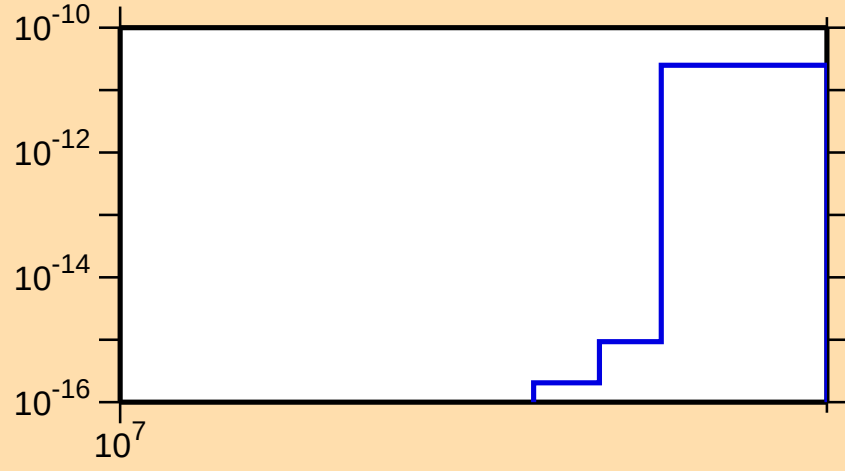
\sigma vs. E for ^{71}\text{As}(n,\text{pt})
