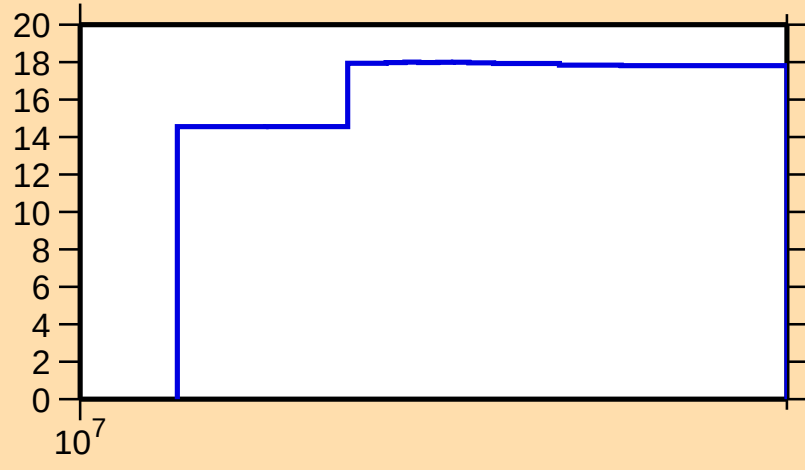
\Delta\sigma/\sigma vs. E for ^{71}\text{As}(n,\text{el.})
