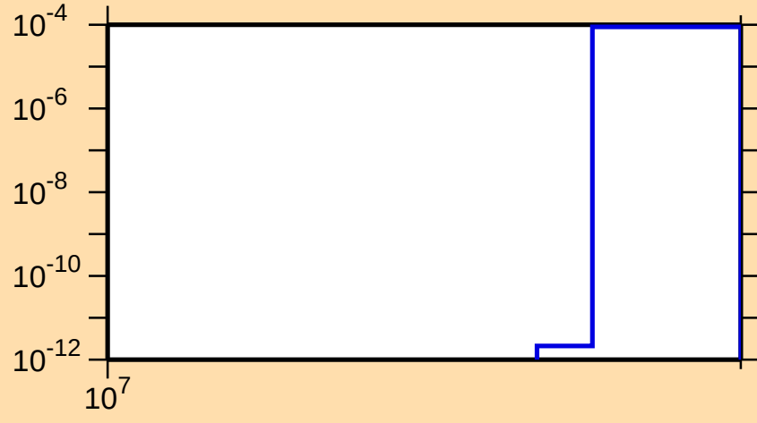
\sigma vs. E for ^{71}\text{As}(n,2np)
