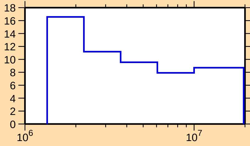
\Delta\sigma/\sigma vs. E for ^{71}\text{As}(n,n\text{oncl.})
