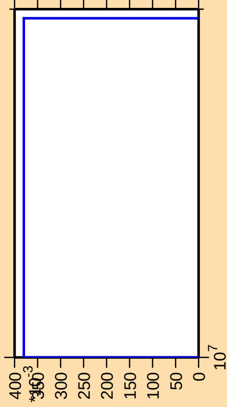
\Delta\sigma/\sigma vs. E for ^{71}\text{As}(n,\text{pt})
