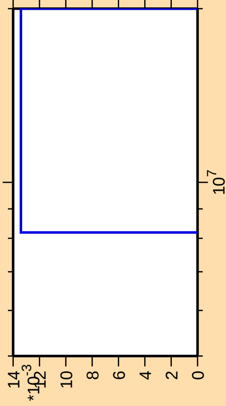
\Delta\sigma/\sigma vs. E for ^{71}\text{As}(\text{mt } 34)
