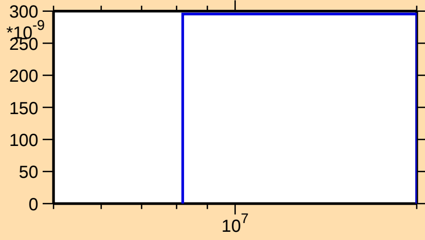
\sigma vs. E for ^{71}\text{As}(n,\text{nd})
