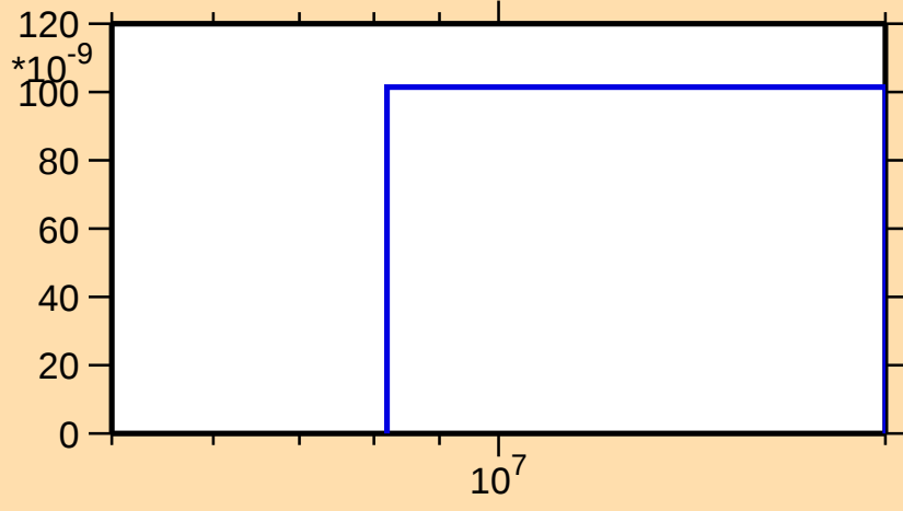
\sigma vs. E for ^{71}\text{As}(\text{mt117})
