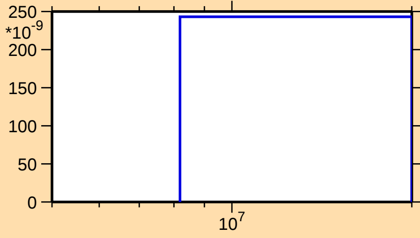
\sigma vs. E for ^{71}\text{As}(\text{mt } 45)
