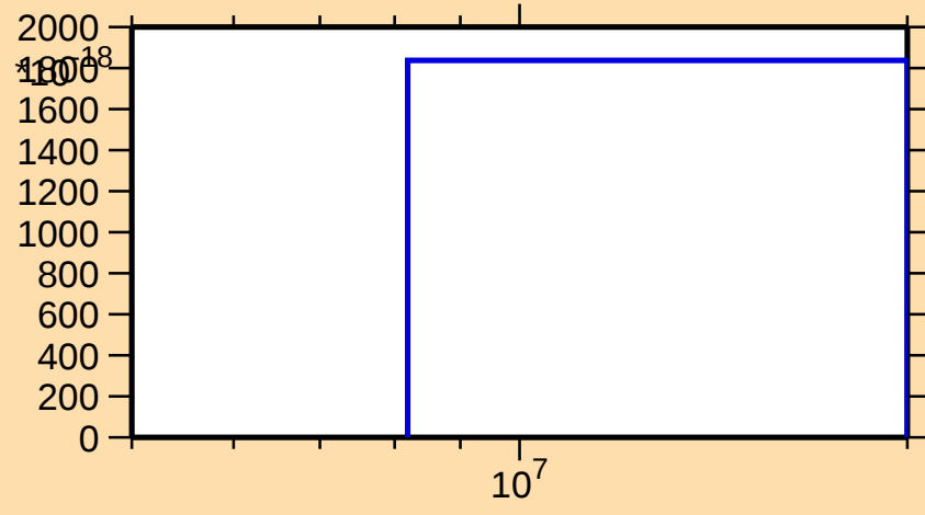
\sigma vs. E for ^{71}\text{As}(\text{mt } 34)
