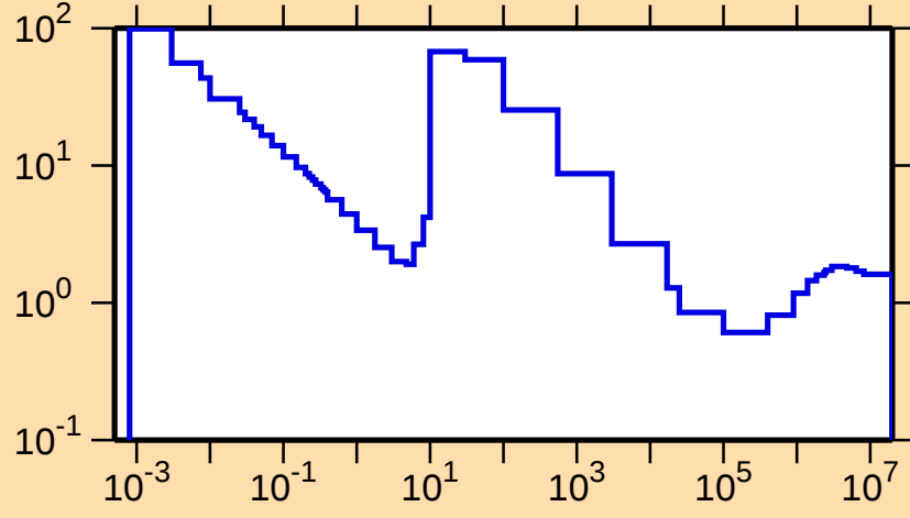
\sigma vs. E for ^{71}\text{As}(n,\text{nonel.})
