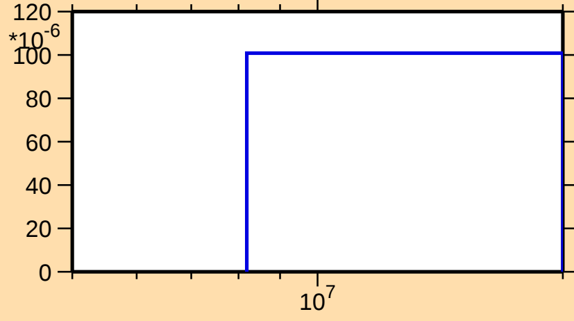
\sigma vs. E for ^{71}\text{As}(n,t)
