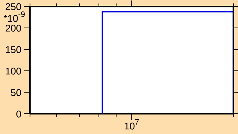
\sigma vs. E for ^{71}\text{As}(n,\text{pd})
