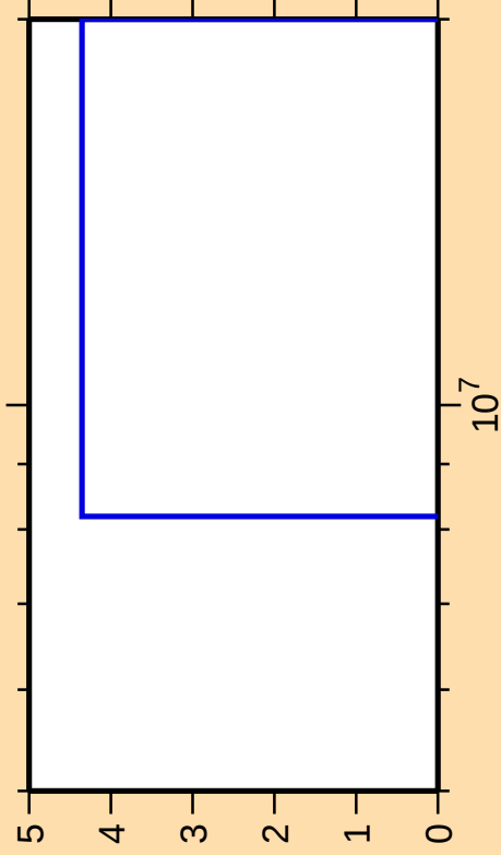
\Delta\sigma/\sigma vs. E for ^{71}\text{As}(n,2n\alpha)
