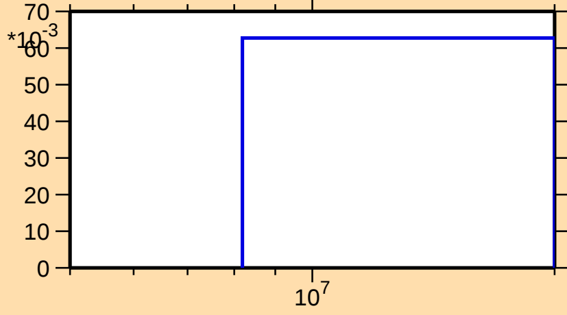
\sigma vs. E for ^{71}\text{As}(n,2n)
