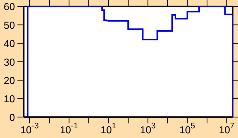
\Delta\sigma/\sigma vs. E for ^{71}\text{As}(n,p)
