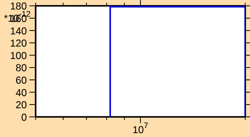
\sigma vs. E for ^{71}\text{As}(n,nt)
