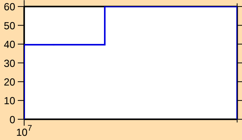
\Delta\sigma/\sigma vs. E for ^{73}\text{As}(n,\text{inel.})
