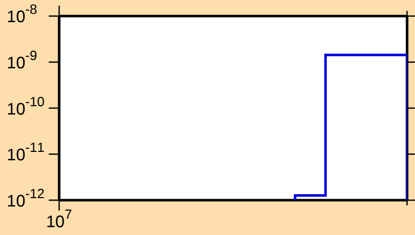
\sigma vs. E for ^{73}\text{As}(n,\text{pd})
