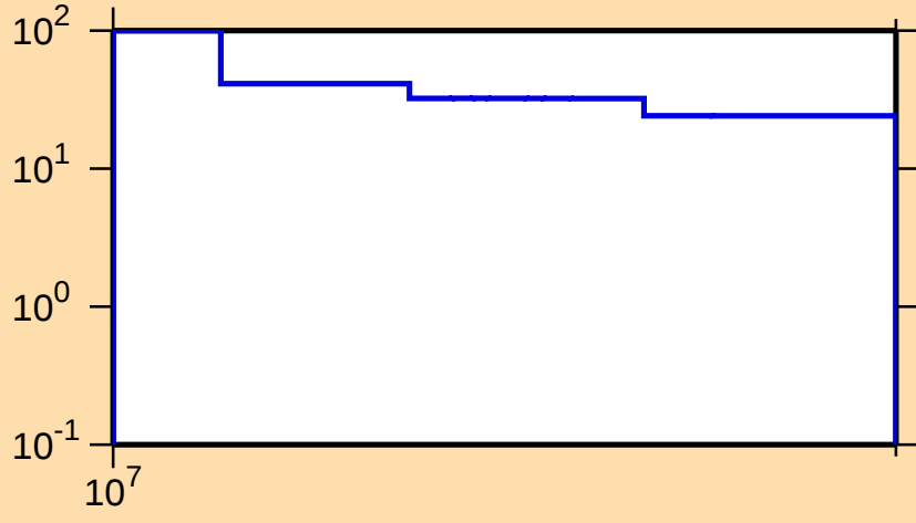
\Delta\sigma/\sigma vs. E for ^{73}\text{As}(n,2n)
