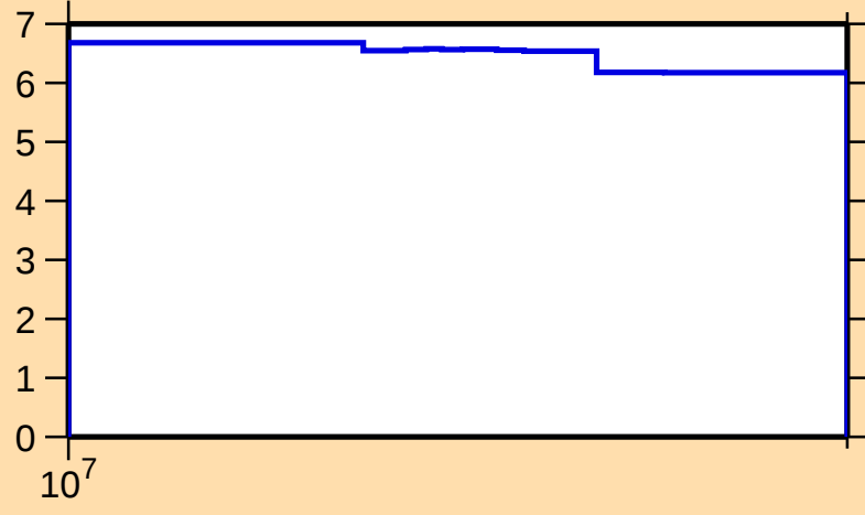
\Delta\sigma/\sigma vs. E for ^{73}\text{As}(n,\text{nonel.})
