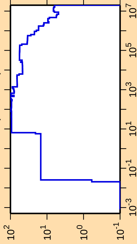
\Delta\sigma/\sigma vs. E for ^{73}\text{As}(n,\text{nonel.})
