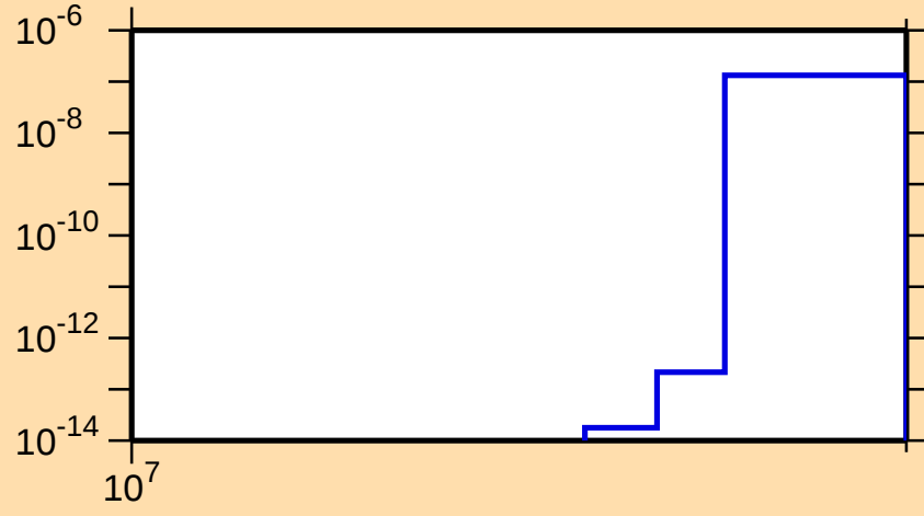
\sigma vs. E for ^{73}\text{As}(n,nt)
