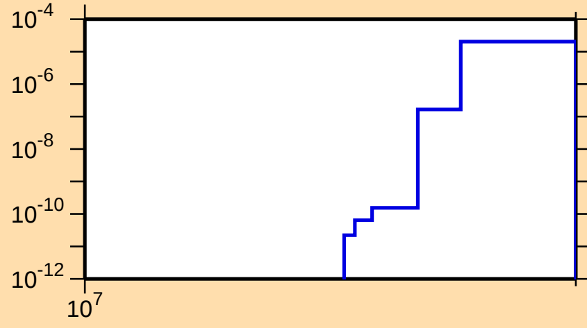
\sigma vs. E for ^{73}\text{As}(n,\text{nd})
