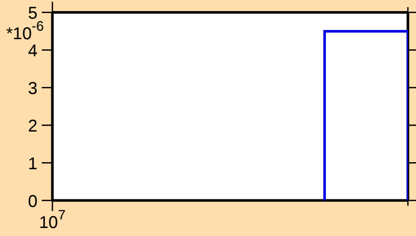
\sigma vs. E for ^{73}\text{As}(n,3n)
