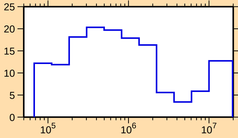
\Delta\sigma/\sigma vs. E for ^{73}\text{As}(n,\text{tot.})
