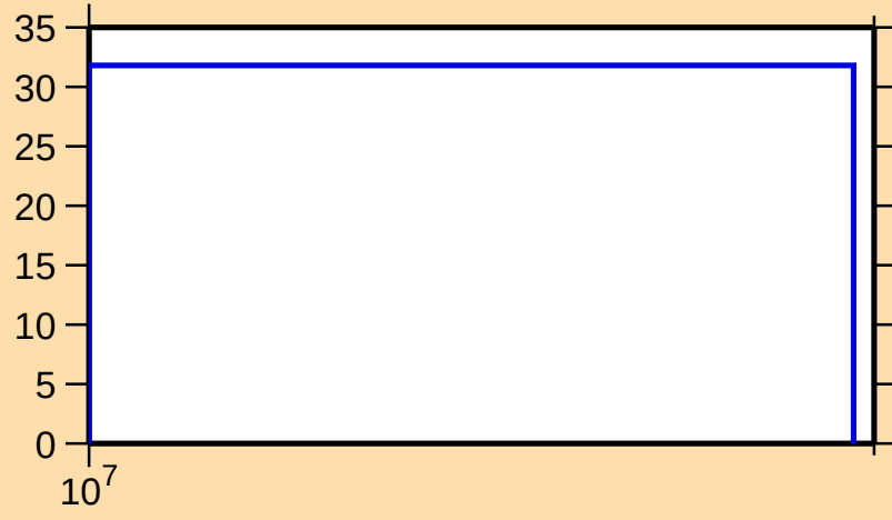
\Delta\sigma/\sigma vs. E for ^{73}\text{As}(n,2n)
