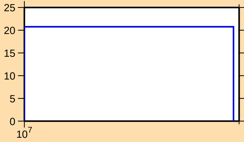
\Delta\sigma/\sigma vs. E for ^{73}\text{As}(n,\text{el.})
