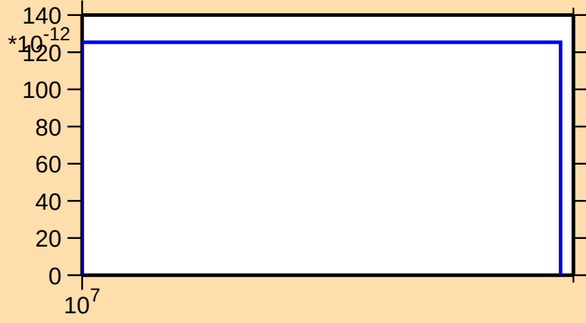
\sigma vs. E for ^{73}\text{As}(\text{mt117})
