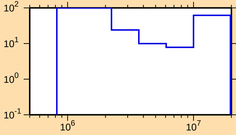
\Delta\sigma/\sigma vs. E for ^{73}\text{As}(n,ncont.)
