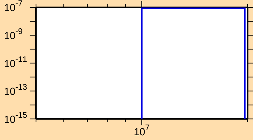
\sigma vs. E for ^{73}\text{As}(n,\text{He3})
