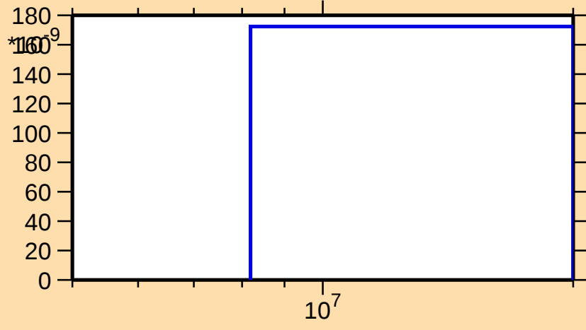
\sigma vs. E for ^{73}\text{As}(n,\text{nd})
