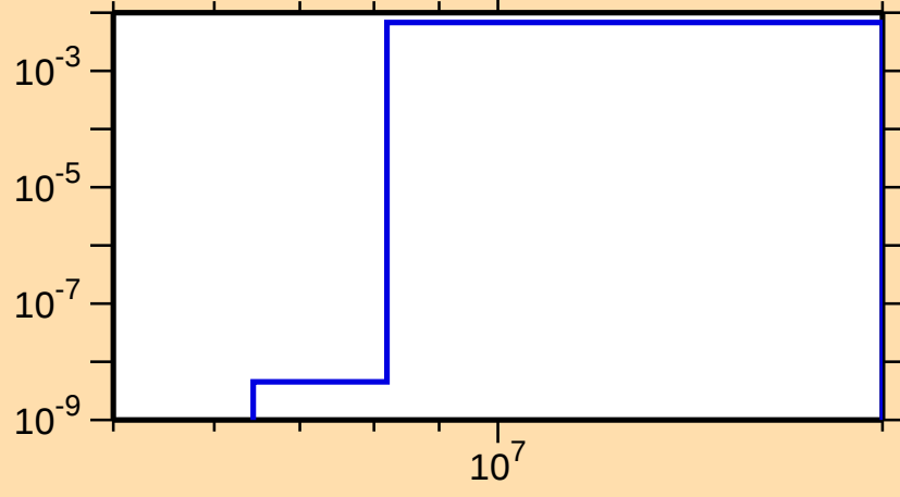
\sigma vs. E for ^{73}\text{As}(n,n\alpha)
