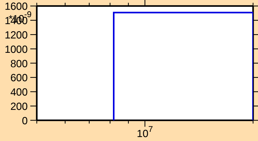
\sigma vs. E for ^{73}\text{As}(n,p\alpha)
