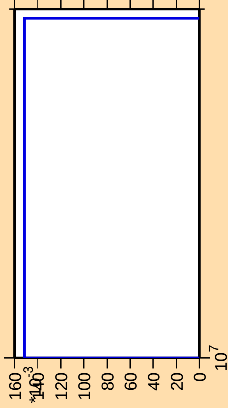
\Delta\sigma/\sigma vs. E for ^{74}\text{As}(n,\text{pd})
