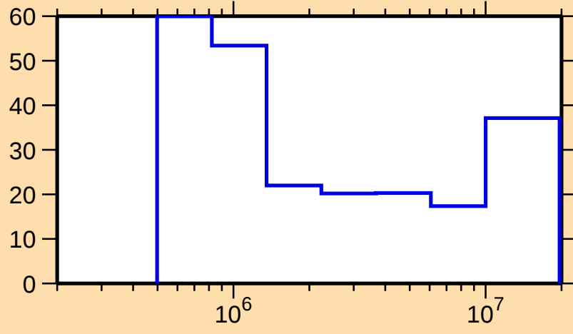
\Delta\sigma/\sigma vs. E for ^{74}\text{As}(n,n\text{cont.})
