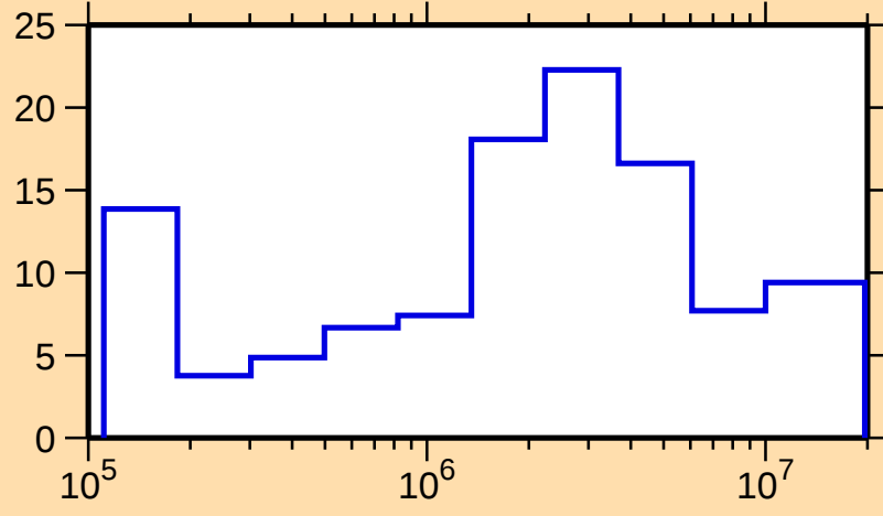
\Delta\sigma/\sigma vs. E for ^{74}\text{As}(\text{n,el.})
