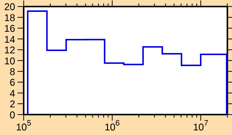
\Delta\sigma/\sigma vs. E for ^{74}\text{As}(\text{n,nonel.})
