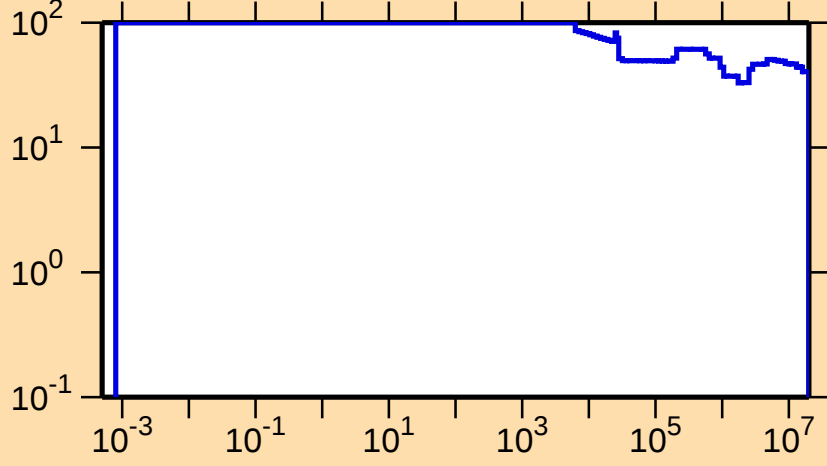
\Delta\sigma/\sigma vs. E for ^{76}\text{As}(n,p)
