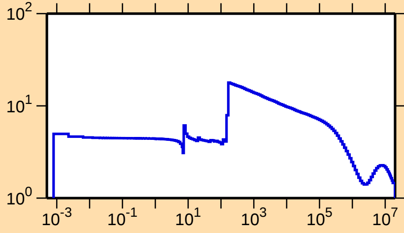
\sigma vs. E for ^{76}\text{As}(n,\text{el.})
