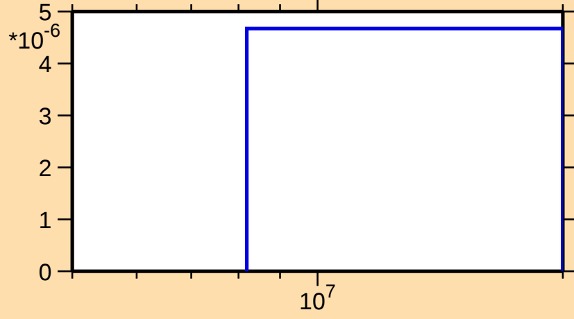
\sigma vs. E for ^{76}\text{As}(n,\text{nd})
