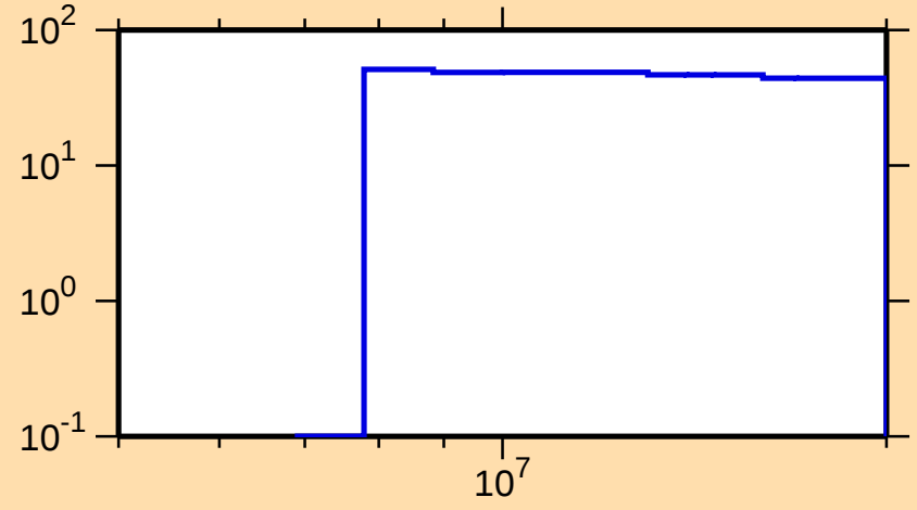
\Delta\sigma/\sigma vs. E for ^{84}\text{As}(n,p)
