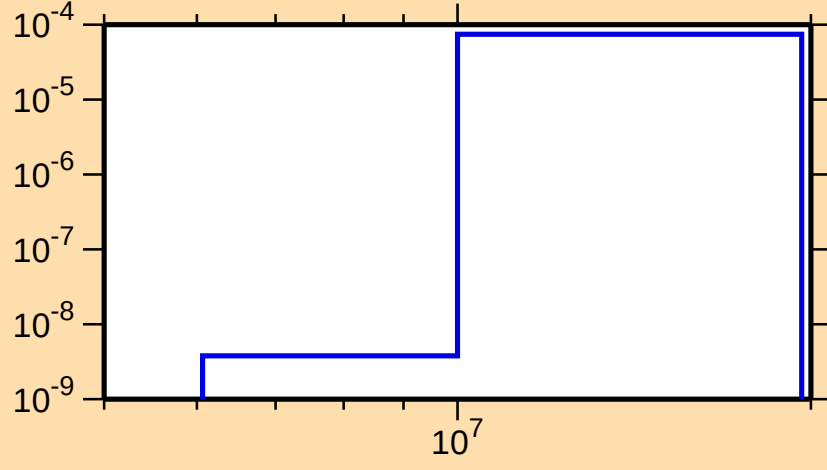
\sigma vs. E for ^{84}\text{As}(n,\alpha)
