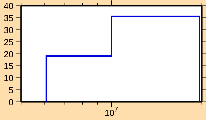
\Delta\sigma/\sigma vs. E for ^{84}\text{As}(n,n\text{cont.})
