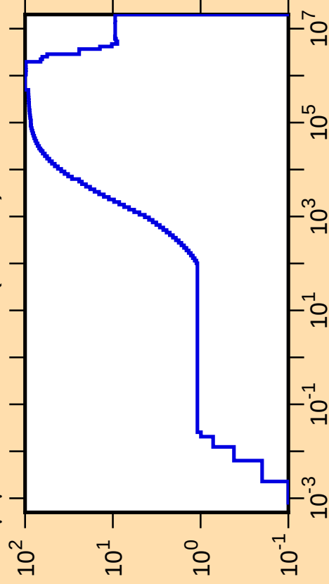
\Delta\mu/\mu vs. E for ^{219}\text{At}(\text{mt251})
