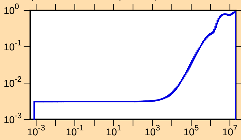
\mu vs. E for ^{219}\text{At}(\text{mt251})
