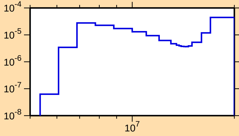
\sigma vs. E for ^{219}\text{At}(n,2n\alpha)
