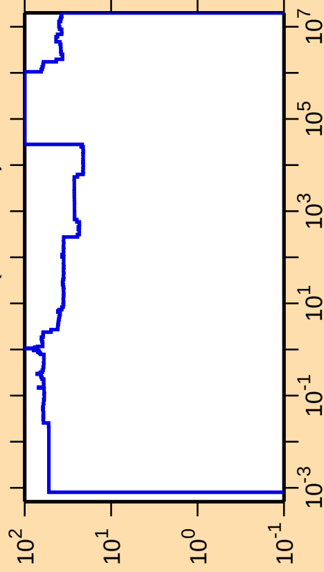
\Delta\sigma/\sigma vs. E for ^{219}\text{At}(n,\text{nonel.})
