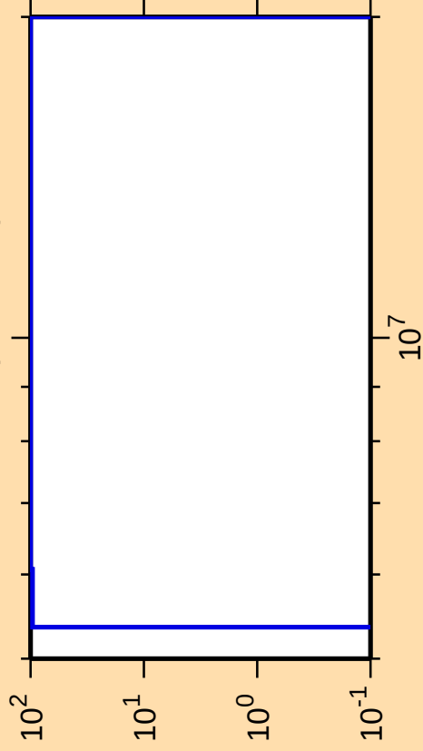
\Delta\sigma/\sigma vs. E for ^{219}\text{At}(n,n\text{cont.})
