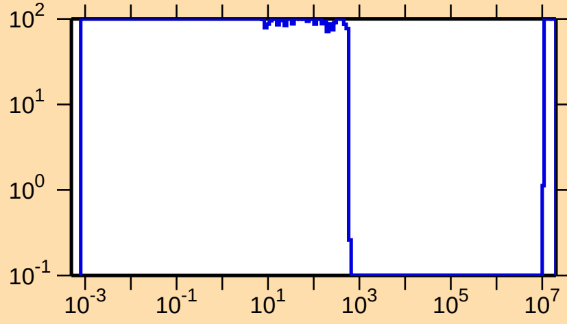
\Delta\sigma/\sigma vs. E for ^{219}\text{At}(n,f)
