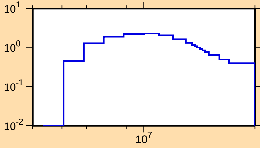
\sigma vs. E for ^{219}\text{At}(n,2n)
