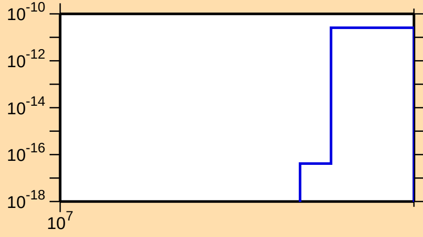
\sigma vs. E for ^{219}\text{At}(\text{mt } 42)
