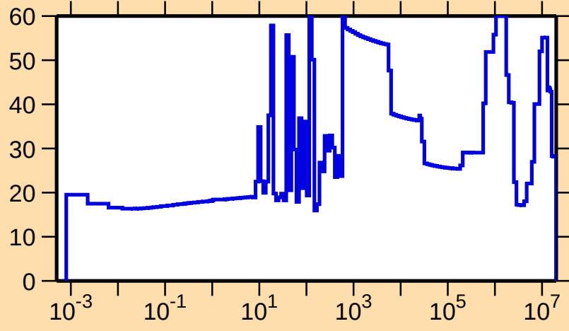
\Delta\sigma/\sigma vs. E for ^{219}\text{At}(n,\text{tot.})
