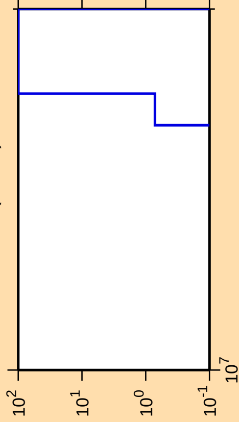
\Delta\sigma/\sigma vs. E for ^{219}\text{At}(\text{mt } 11)
