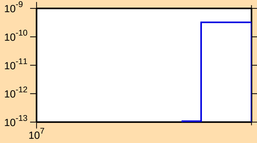
\sigma vs. E for ^{219}\text{At}(\text{mt } 11)
