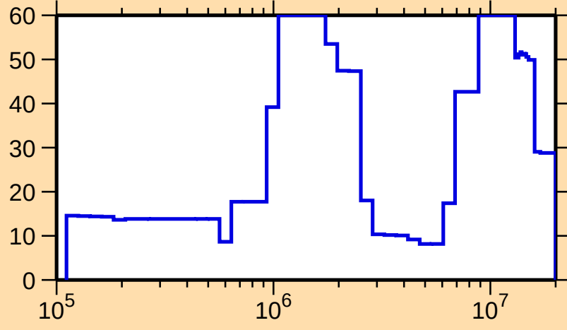
\Delta\sigma/\sigma vs. E for ^{219}\text{At}(n,\text{el.})
