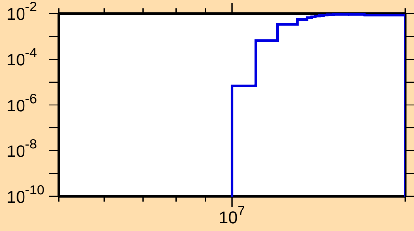
\sigma vs. E for ^{219}\text{At}(n,3n\alpha)
