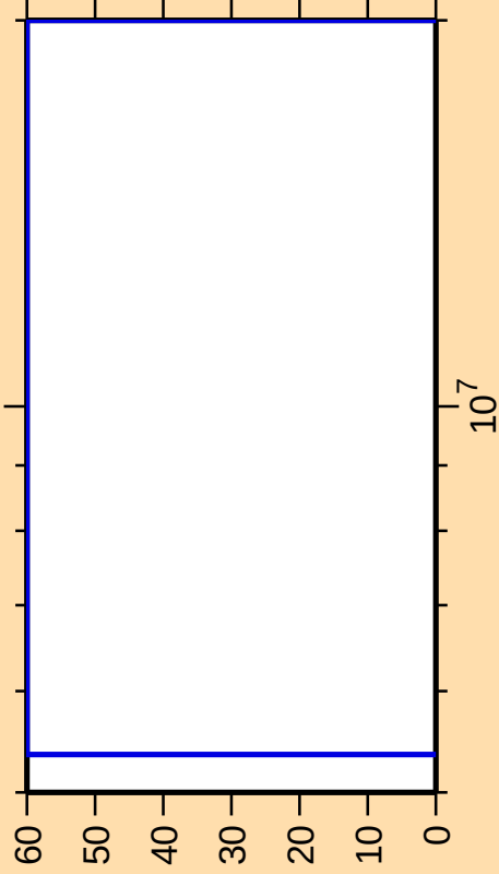
\Delta\sigma/\sigma vs. E for ^{219}\text{At}(n,2n)
