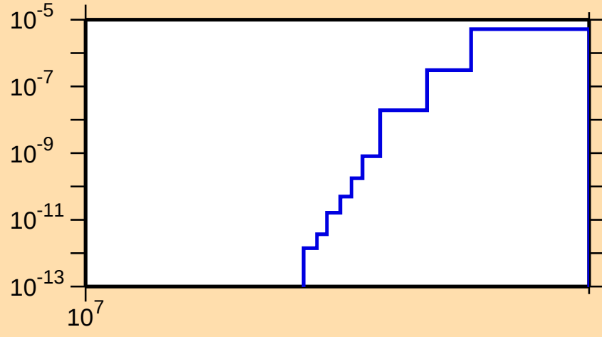
\sigma vs. E for ^{219}\text{At}(n,2np)
