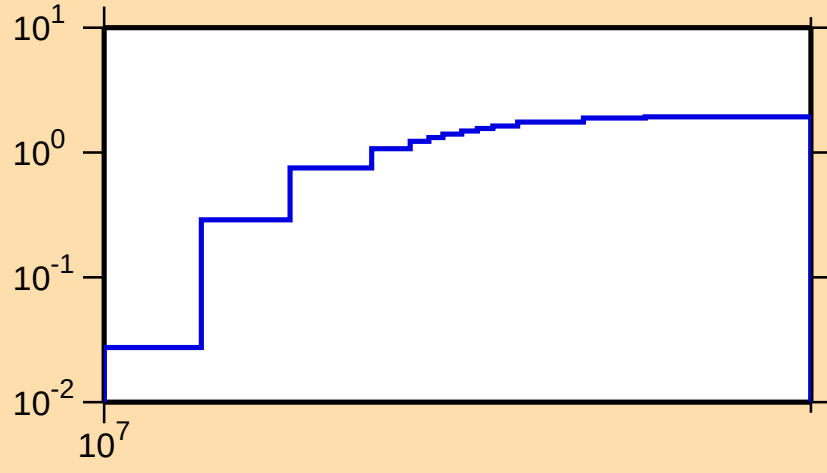
\sigma vs. E for ^{219}\text{At}(n,3n)
