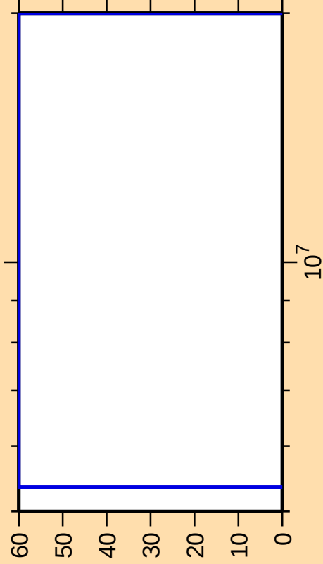
\Delta\sigma/\sigma vs. E for ^{219}\text{At}(n,2n\alpha)
