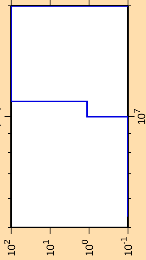
\Delta\sigma/\sigma vs. E for ^{219}\text{At}(n,f)
