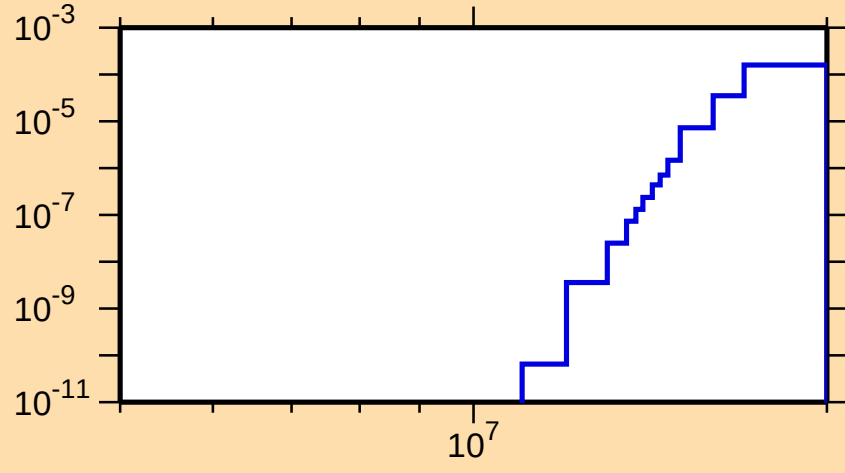
\sigma vs. E for ^{219}\text{At}(n,nt)
