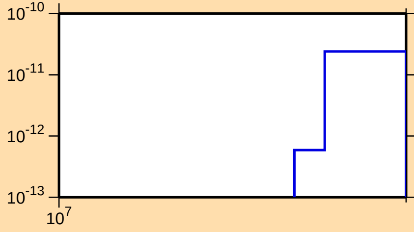
\sigma vs. E for ^{219}\text{At}(n,\text{He3})
