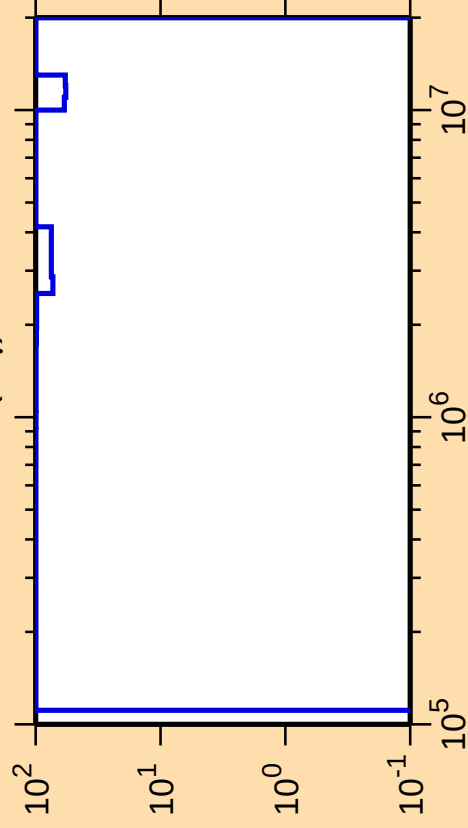
\Delta\sigma/\sigma vs. E for ^{219}\text{At}(n,\gamma)
