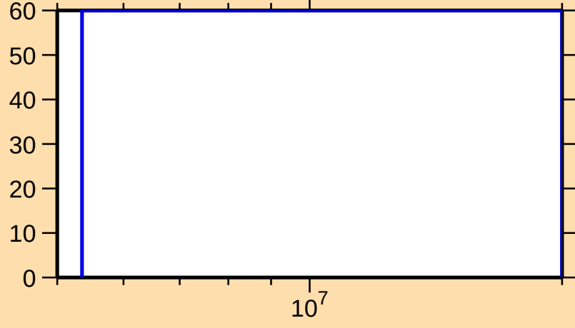
\Delta\sigma/\sigma vs. E for ^{219}\text{At}(n,2n)
