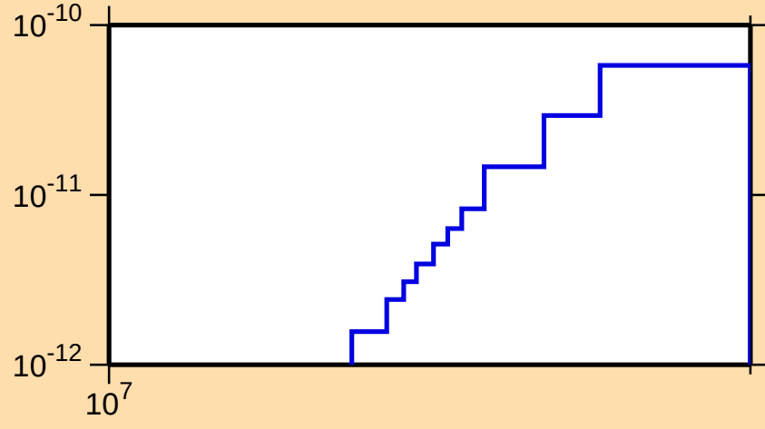
\sigma vs. E for ^{219}\text{At}(n,p\alpha)
