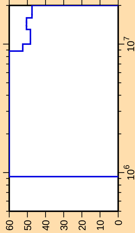
\Delta\sigma/\sigma vs. E for ^{219}\text{At}(n,n\alpha)
