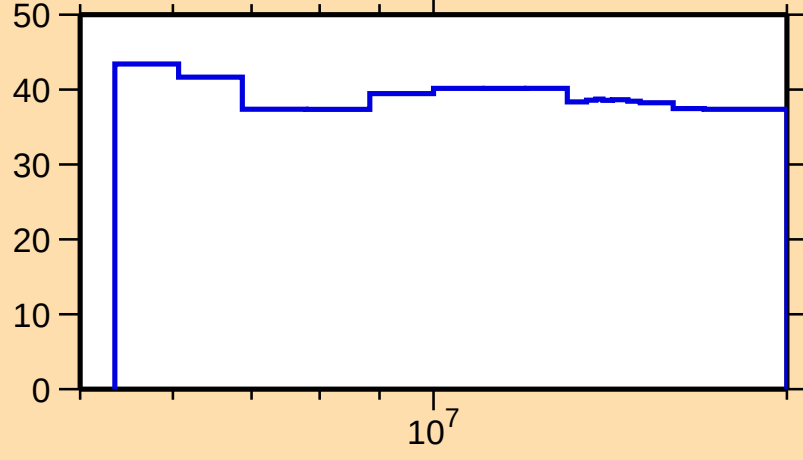
\Delta\sigma/\sigma vs. E for ^{219}\text{At}(n,\text{nonel.})
