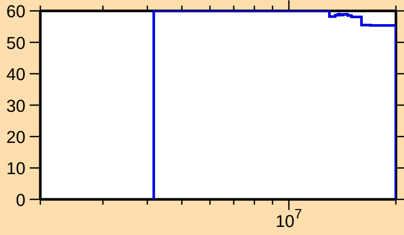
\Delta\sigma/\sigma vs. E for ^{219}\text{At}(n,n_1)
