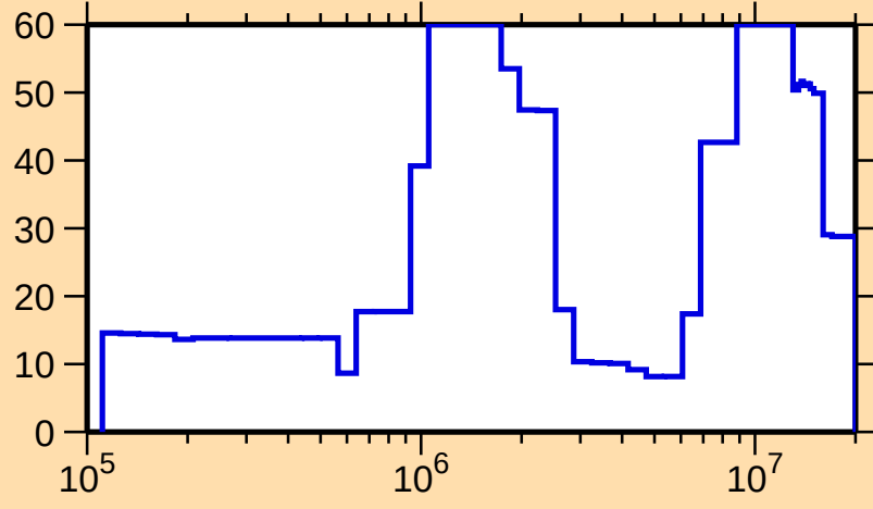
\Delta\sigma/\sigma vs. E for ^{219}\text{At}(n,\text{el.})
