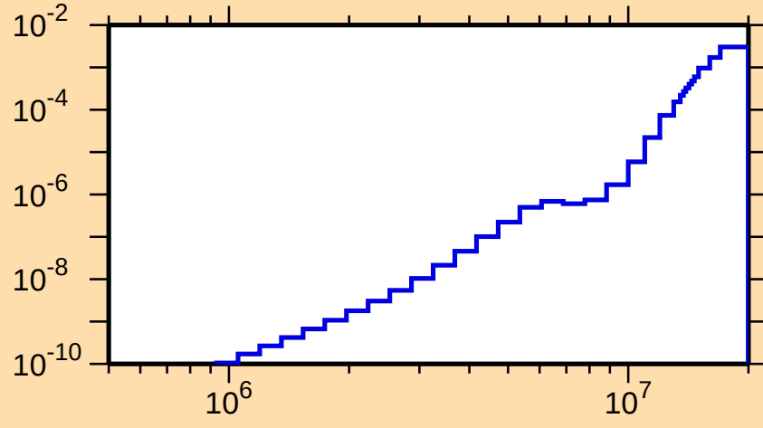
\sigma vs. E for ^{219}\text{At}(n,n\alpha)
