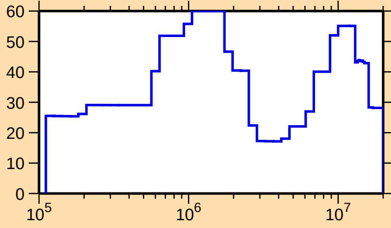
\Delta\sigma/\sigma vs. E for ^{219}\text{At}(n,\text{tot.})
