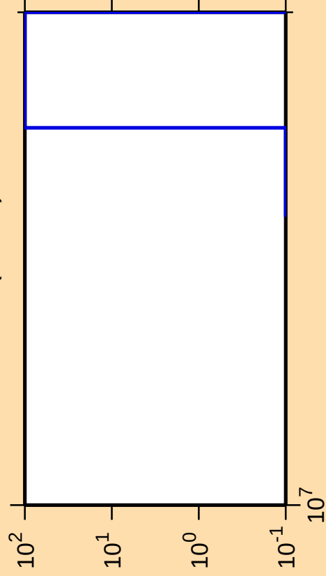
\Delta\sigma/\sigma vs. E for ^{219}\text{At}(\text{mt } 42)
