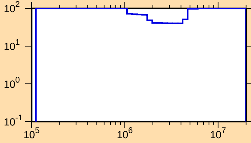
\Delta\sigma/\sigma vs. E for ^{219}\text{At}(n,\text{inel.})
