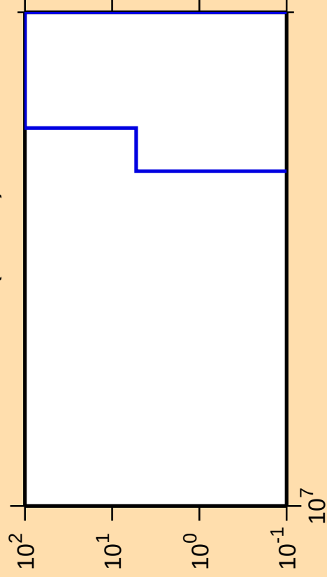
\Delta\sigma/\sigma vs. E for ^{219}\text{At}(n,\text{He3})
