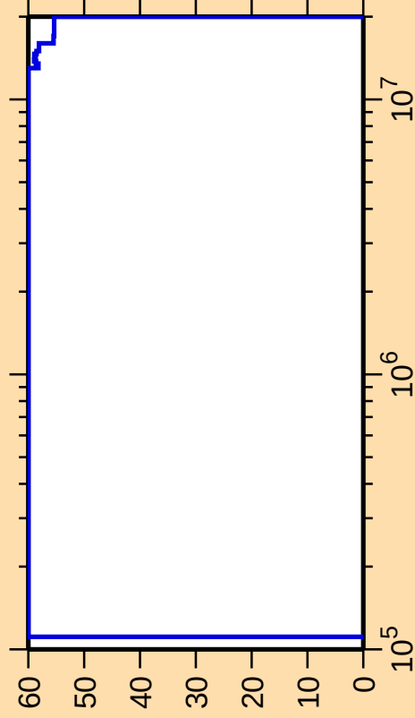
\Delta\sigma/\sigma vs. E for ^{219}\text{At}(n,n_1)
