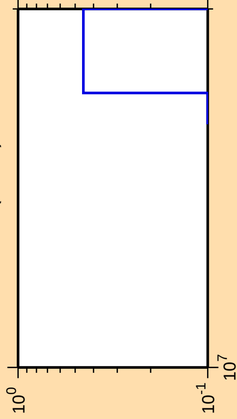
\Delta\sigma/\sigma vs. E for ^{220}\text{At}(\text{mt } 34)
