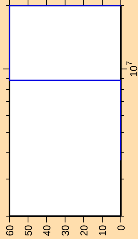
\Delta\sigma/\sigma vs. E for ^{220}\text{At}(n,f)
