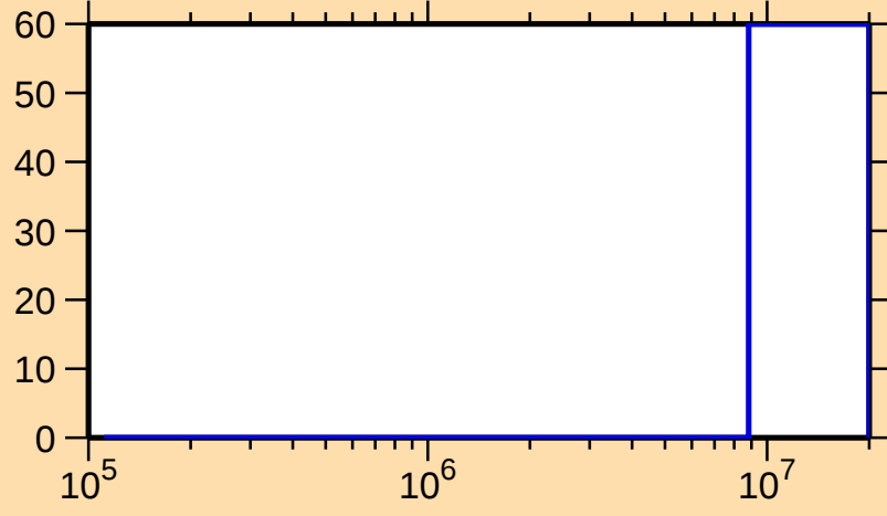
\Delta\sigma/\sigma vs. E for ^{220}\text{At}(n,f)
