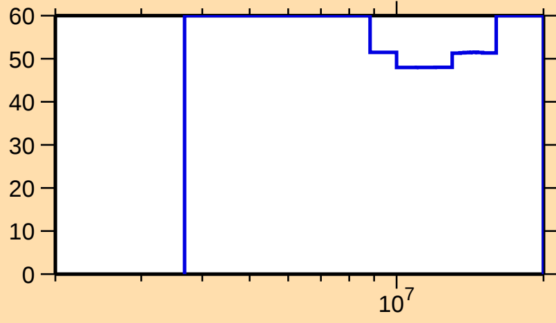
\Delta\sigma/\sigma vs. E for ^{220}\text{At}(n,2n)
