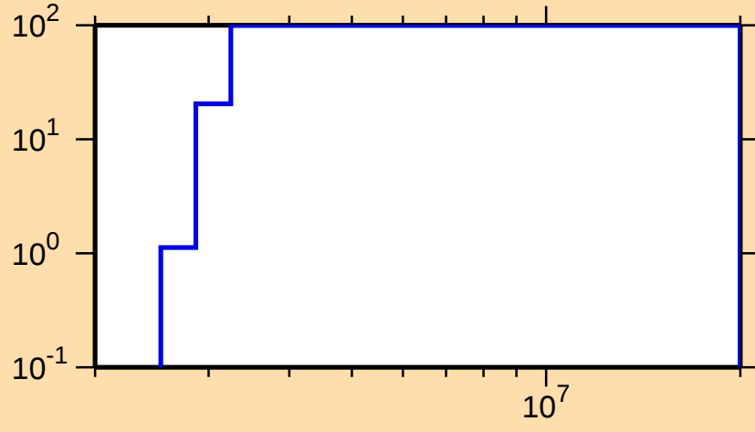
\Delta\sigma/\sigma vs. E for ^{220}\text{At}(n,p)
