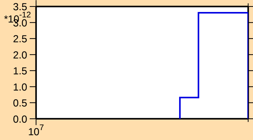
\sigma vs. E for ^{220}\text{At}(\text{mt } 45)
