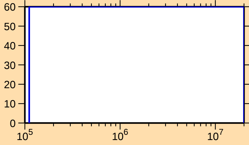
\Delta\sigma/\sigma vs. E for ^{220}\text{At}(n,n_1)
