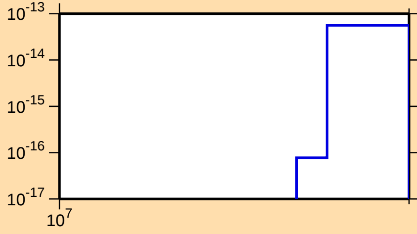
\sigma vs. E for ^{220}\text{At}(\text{mt } 34)
