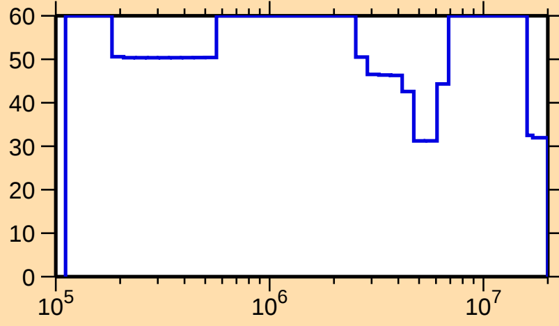
\Delta\sigma/\sigma vs. E for ^{220}\text{At}(n,\text{el.})
