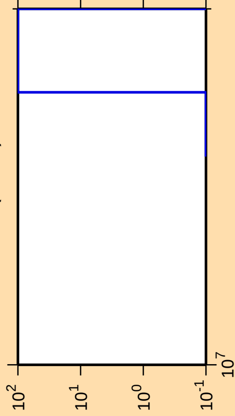
\Delta\sigma/\sigma vs. E for ^{220}\text{At}(\text{mt } 42)
