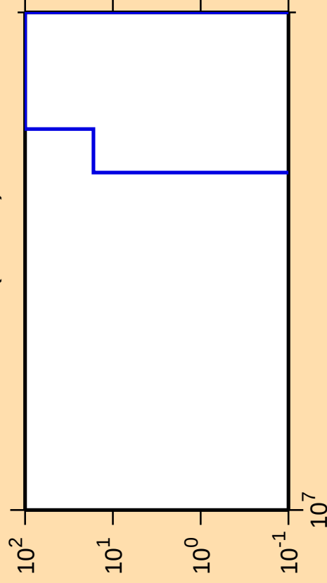
\Delta\sigma/\sigma vs. E for ^{220}\text{At}(n,\text{He3})
