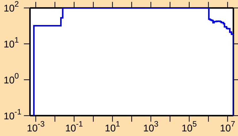
\Delta\sigma/\sigma vs. E for ^{220}\text{At}(n,\text{nonel.})
