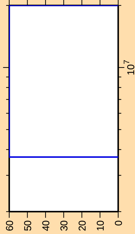
\Delta\sigma/\sigma vs. E for ^{220}\text{At}(n,\gamma)
