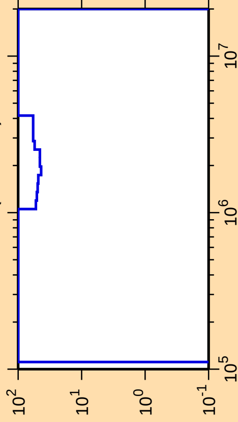
\Delta\sigma/\sigma vs. E for ^{220}\text{At}(n,n\text{cont.})
