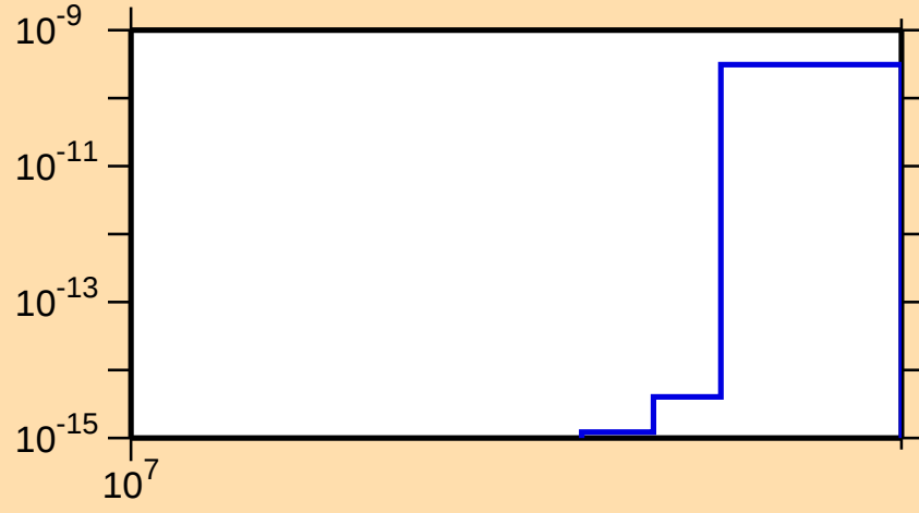
\sigma vs. E for ^{220}\text{At}(\text{mt } 42)
