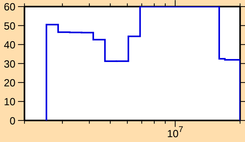
\Delta\sigma/\sigma vs. E for ^{220}\text{At}(n,\text{el.})
