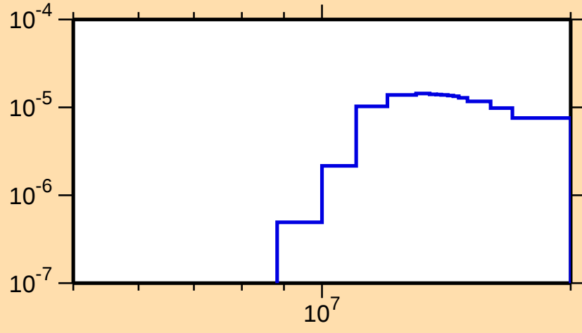
\sigma vs. E for ^{220}\text{At}(n,3n\alpha)
