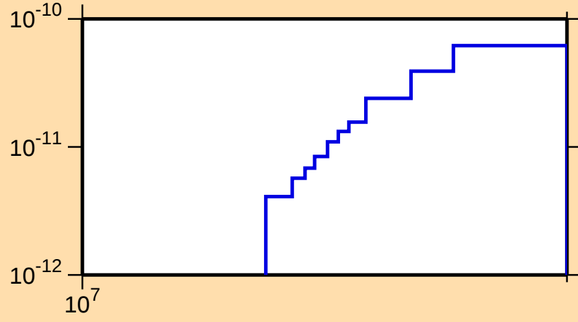
\sigma vs. E for ^{220}\text{At}(n,p\alpha)
