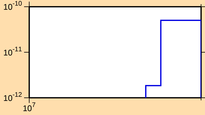
\sigma vs. E for ^{220}\text{At}(n,\text{He3})
