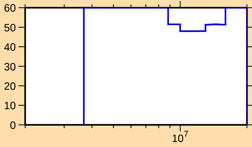
\Delta\sigma/\sigma vs. E for ^{220}\text{At}(n,2n)
