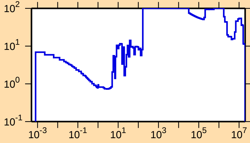
\Delta\sigma/\sigma vs. E for ^{220}\text{At}(n,\text{tot.})
