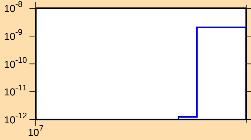
\sigma vs. E for ^{220}\text{At}(\text{mt } 11)
