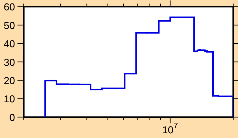
\Delta\sigma/\sigma vs. E for ^{220}\text{At}(n,\text{tot.})
