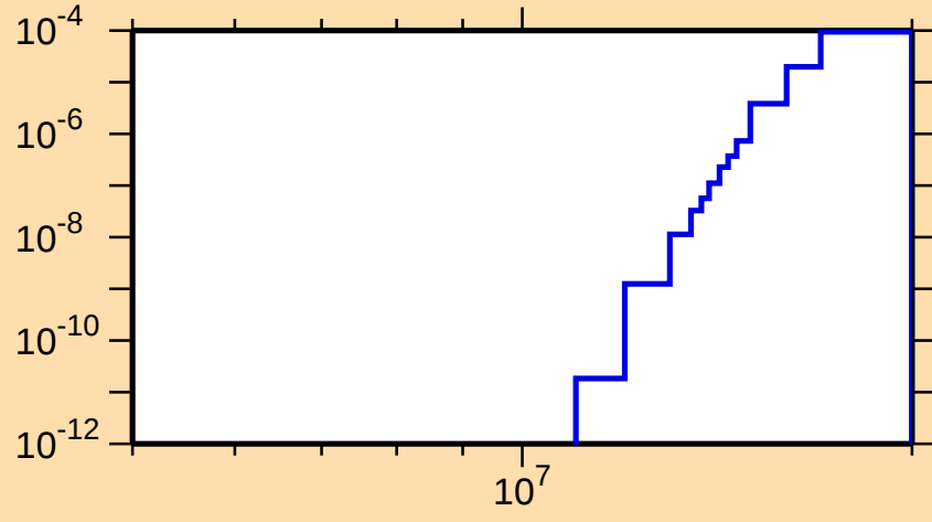
\sigma vs. E for ^{220}\text{At}(n,\text{nd})
