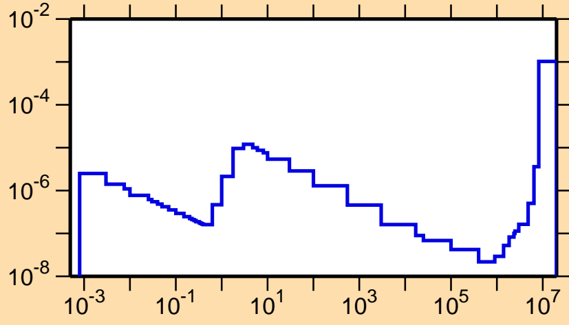
\sigma vs. E for ^{220}\text{At}(n,\alpha)
