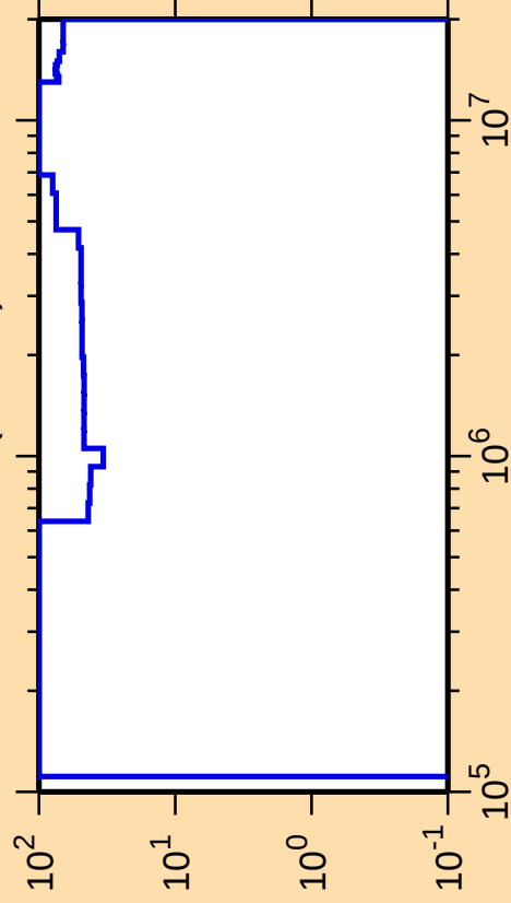
\Delta\sigma/\sigma vs. E for ^{223}\text{At}(n,\text{inel.})
