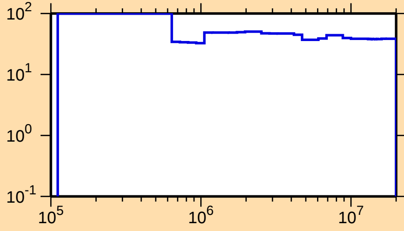
\Delta\sigma/\sigma vs. E for ^{223}\text{At}(n,n\text{nonel.})
