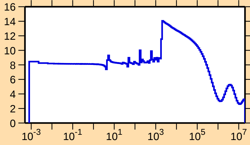
\sigma vs. E for ^{223}\text{At}(n,\text{el.})
