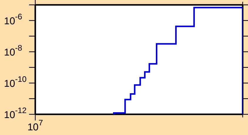
\sigma vs. E for ^{223}\text{At}(n,\text{nd})
