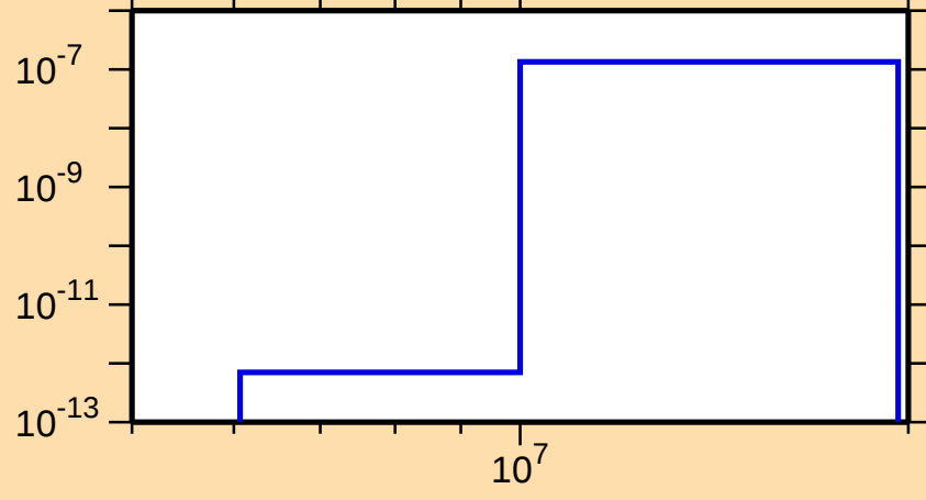
\sigma vs. E for ^{223}\text{At}(n,2n\alpha)
