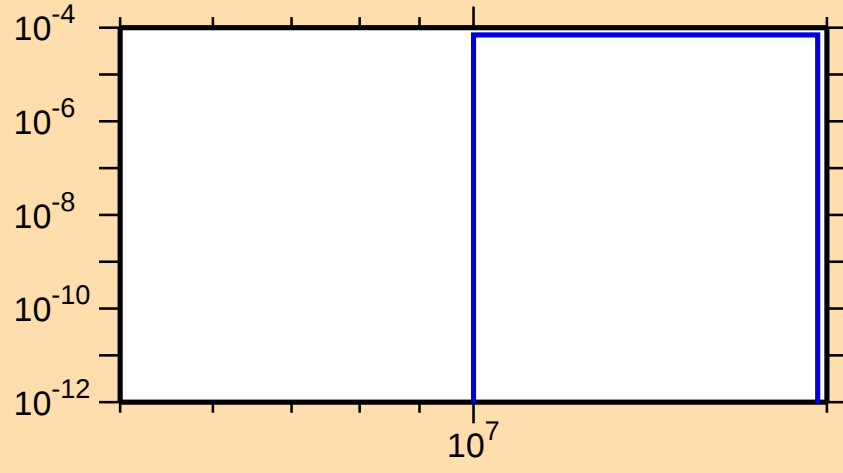
\sigma vs. E for ^{223}\text{At}(n,np)
