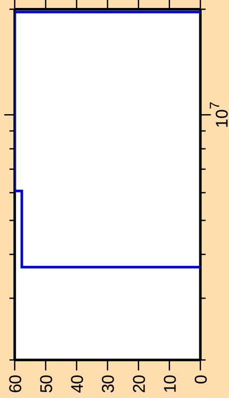
\Delta\sigma/\sigma vs. E for ^{223}\text{At}(n,n\text{cont.})
