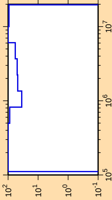
\Delta\sigma/\sigma vs. E for ^{223}\text{At}(n,\text{ncont.})
