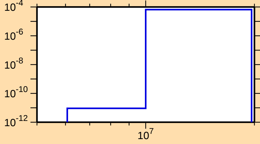
\sigma vs. E for ^{223}\text{At}(n,t)
