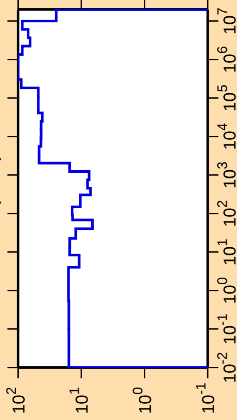
\Delta\sigma/\sigma vs. E for ^{223}\text{At}(n,\text{el.})
