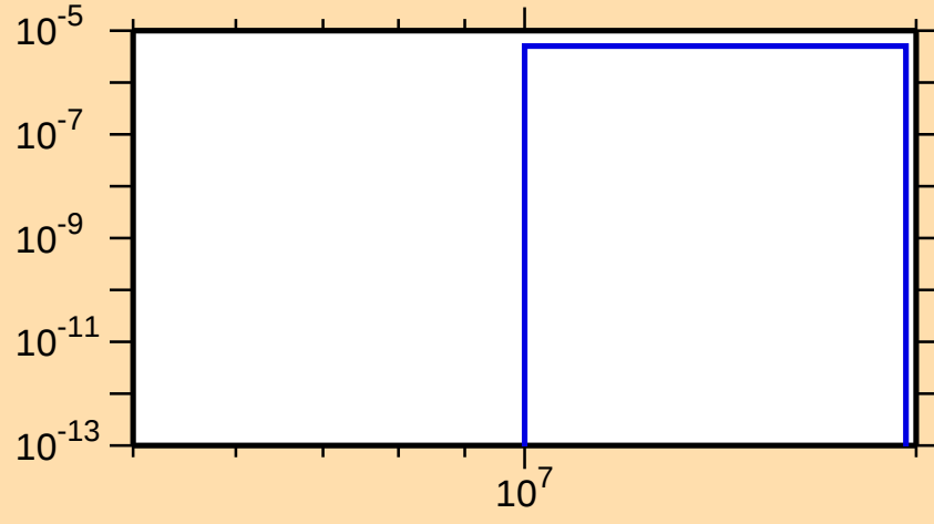
\sigma vs. E for ^{223}\text{At}(n,nt)
