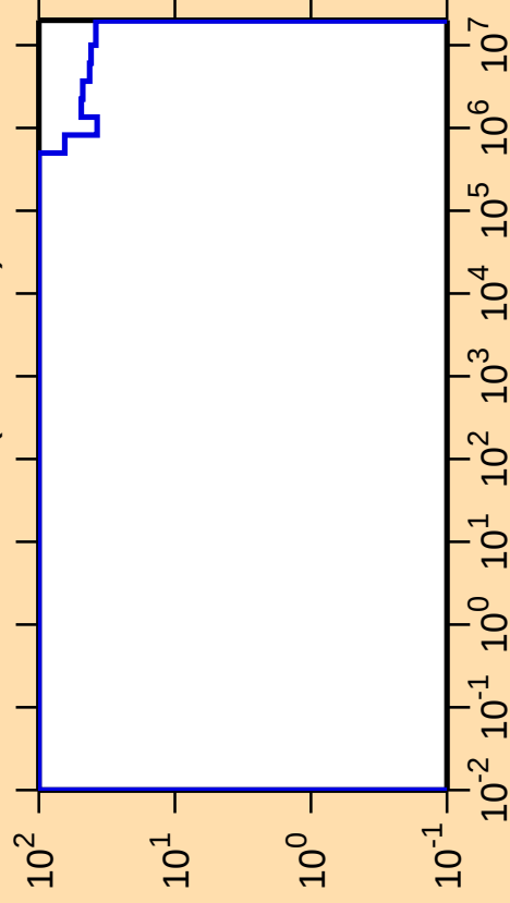
\Delta\sigma/\sigma vs. E for ^{223}\text{At}(n,\text{nonel.})
