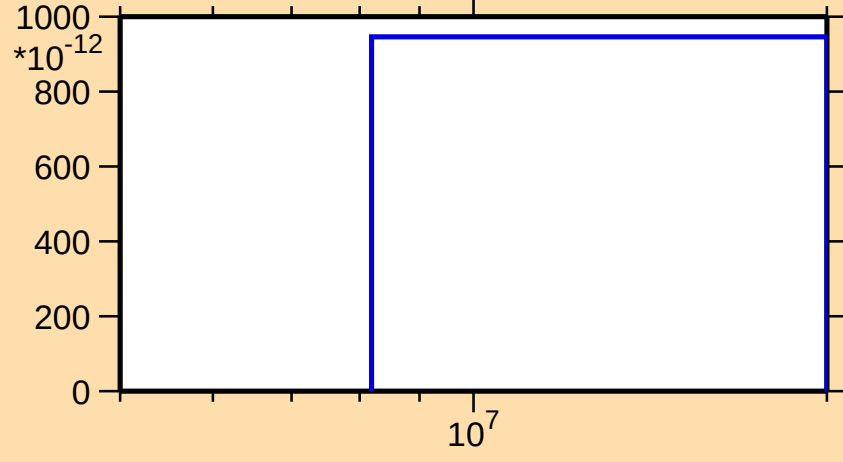
\sigma vs. E for ^{223}\text{At}(n,3n\alpha)
