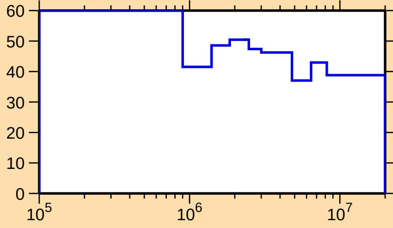
\Delta\sigma/\sigma vs. E for ^{223}\text{At}(n,n\text{onel.})
