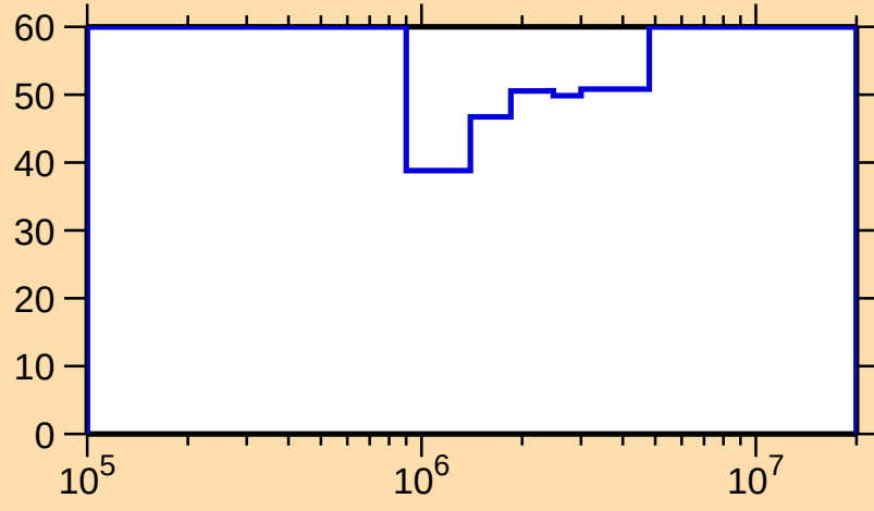
\Delta\sigma/\sigma vs. E for ^{223}\text{At}(n,n\text{cont.})
