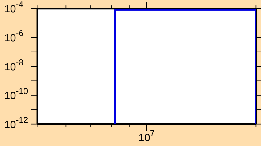
\sigma vs. E for ^{223}\text{At}(n,d)
