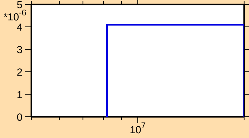
\sigma vs. E for ^{223}\text{At}(n,\text{nt})
