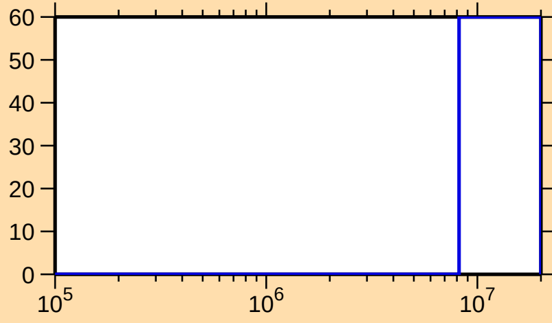
\Delta\sigma/\sigma vs. E for ^{223}\text{At}(n,\text{f})
