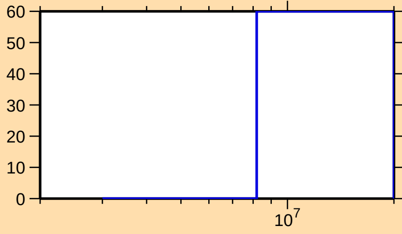
\Delta\sigma/\sigma vs. E for ^{223}\text{At}(n,f)
